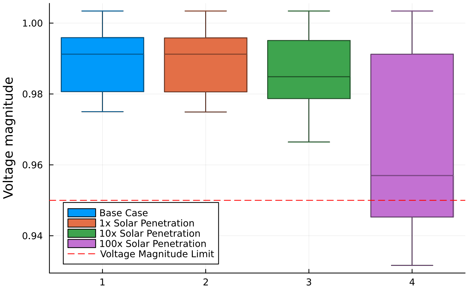
Nodal Voltage Magnitude under the different scenario
