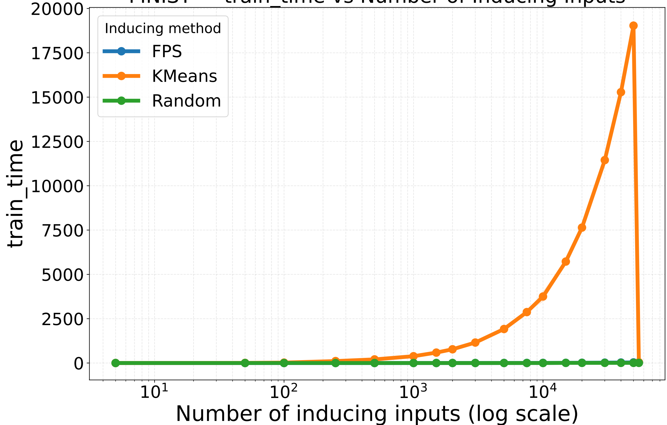
MNIST — train_time vs Number of Inducing Inputs
