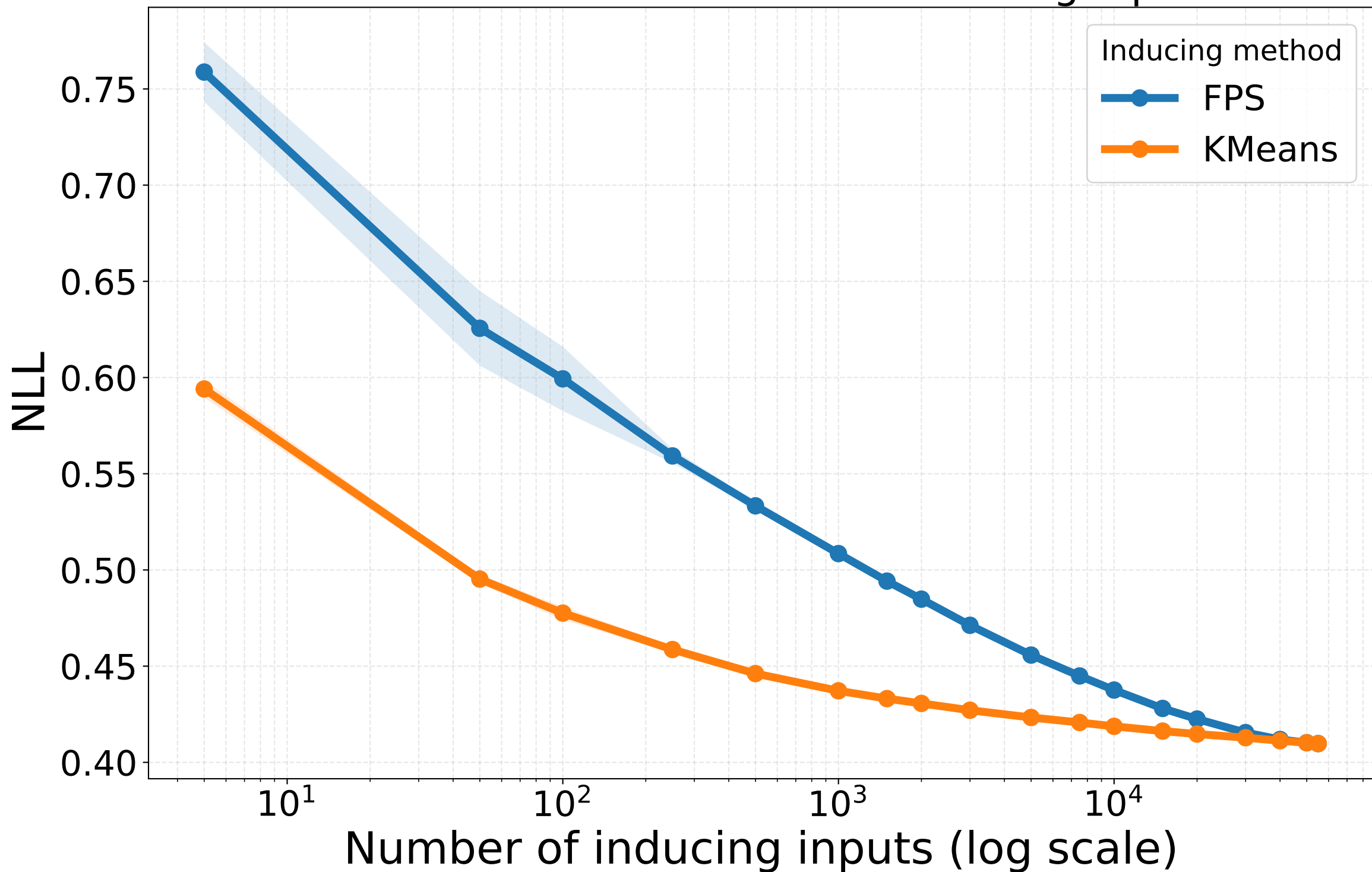
FMNIST — NLL vs Number of Inducing Inputs
