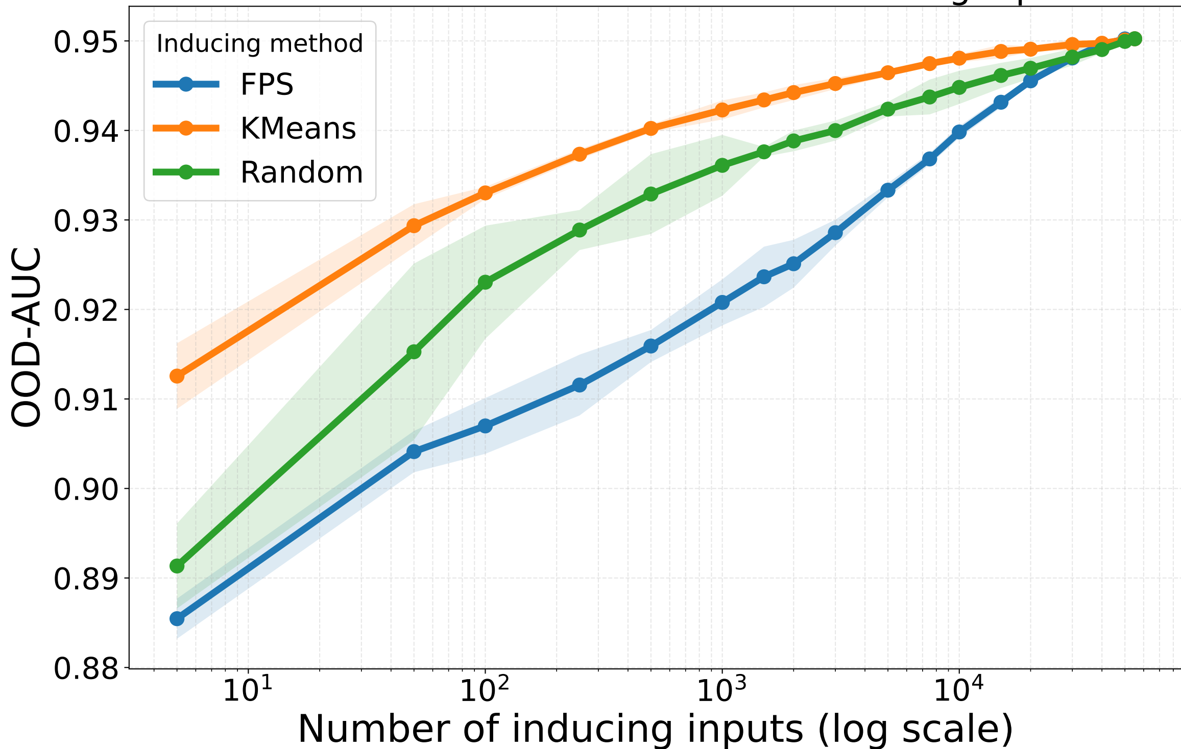
MNIST — OOD-AUC vs Number of Inducing Inputs
