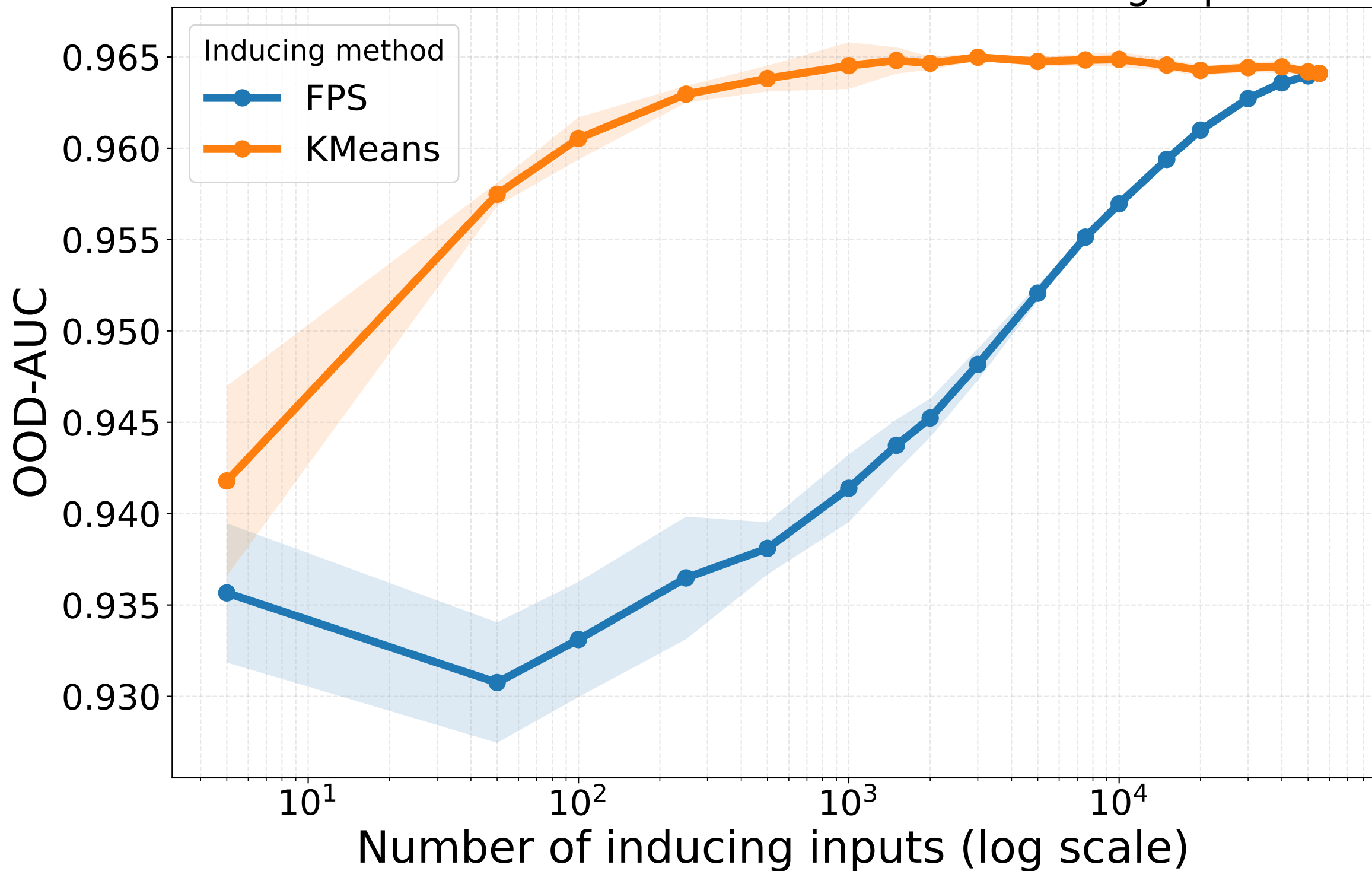
FMNIST — OOD-AUC vs Number of Inducing Inputs
