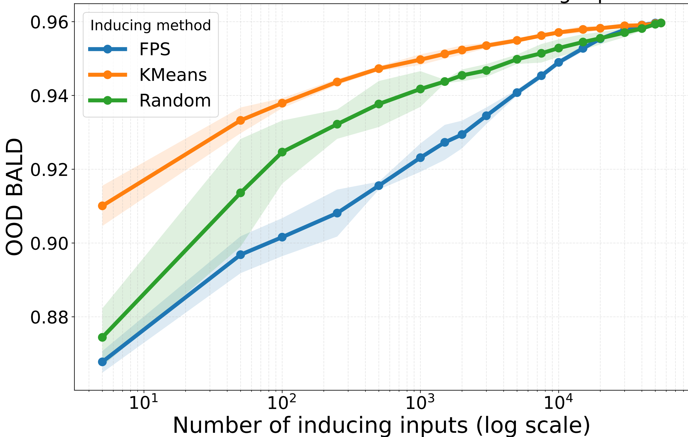
MNIST — OOD BALD vs Number of Inducing Inputs
