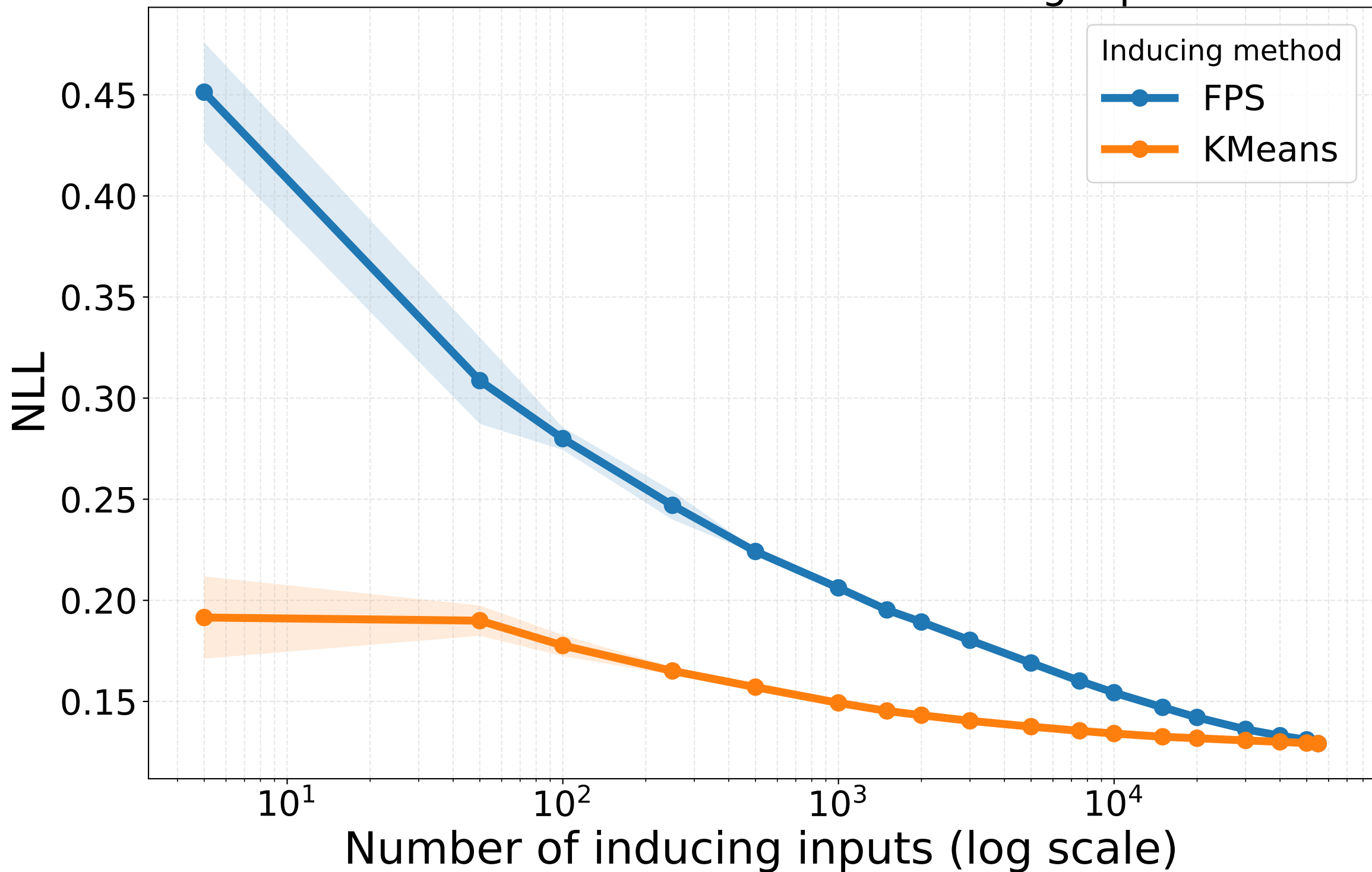
MNIST — NLL vs Number of Inducing Inputs
