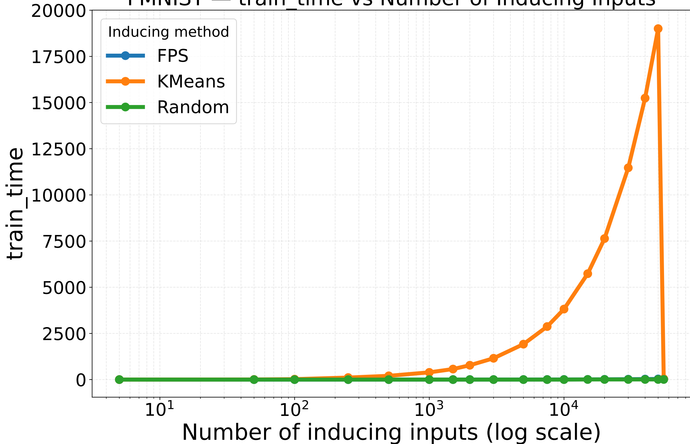
FMNIST — train_time vs Number of Inducing Inputs
