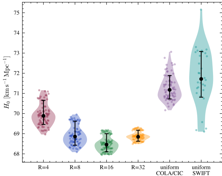
Field-median distribution
