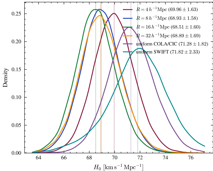
Stacked posteriors
