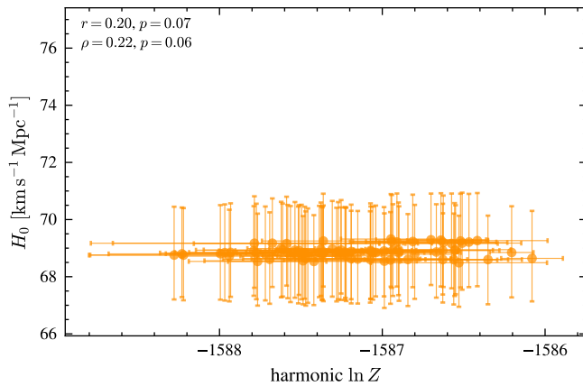
R = 32 h^{-1} \text{Mpc}
