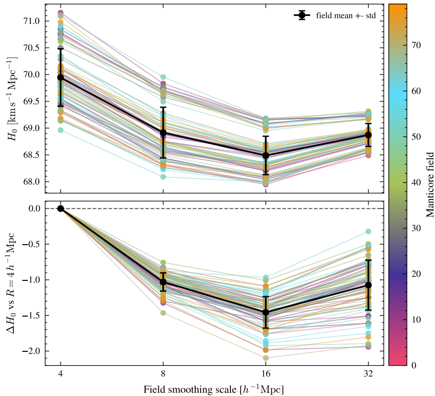
Matched Manticores realisations
