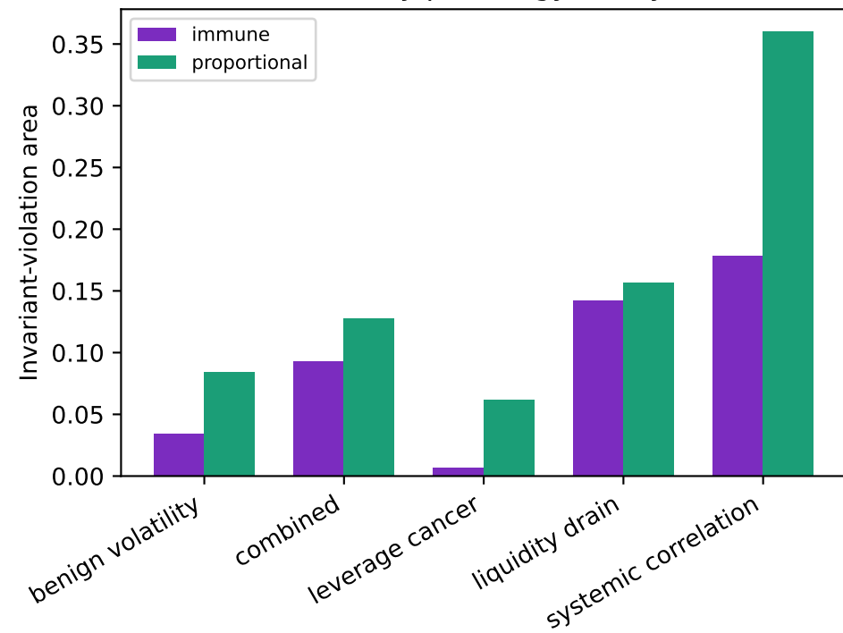
Targeted defense beat proportional in every pathology family
