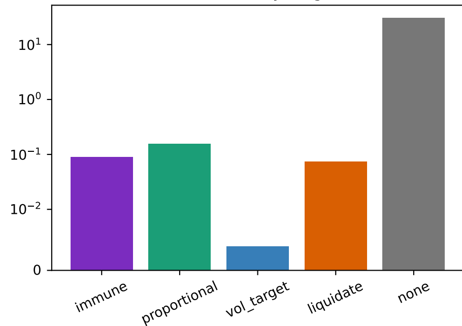
Invariant-violation area (lower is safer; symlog scale)
