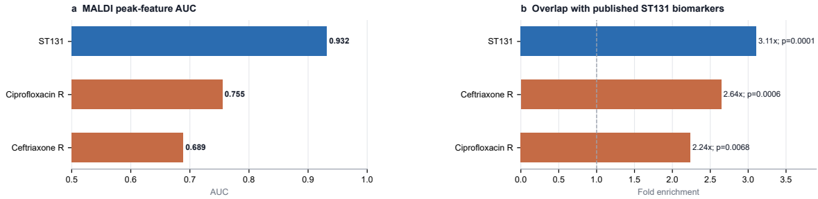
Fig. 5 | Public WGS-linked MALDI data support lineage encoding Public Basel UPEC spectra link MALDI peak features, WGS-derived lineage labels, and resistance phenotypes.
