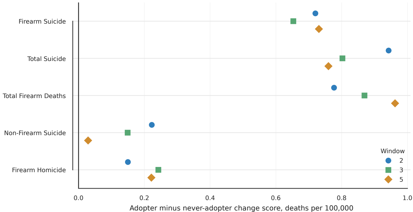
Change-score robustness across pre/post windows
