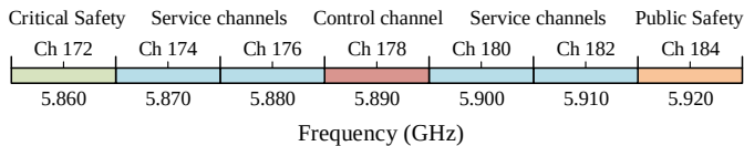
Fig. 20: The frequency channels allocated for DSRC.
