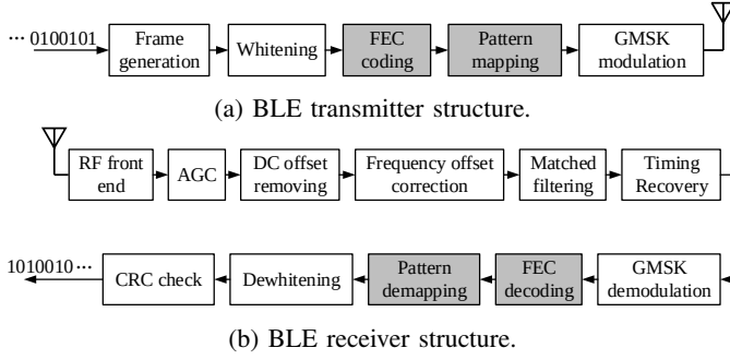
Fig. 16: Signal processing block diagram of Bluetooth communication.
