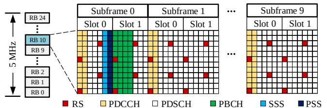
Fig. 8: LTE downlink resource grid [88].
