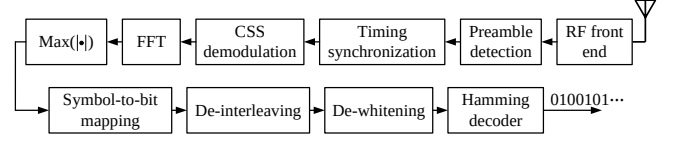
(b) The LoRa receiver structure.
