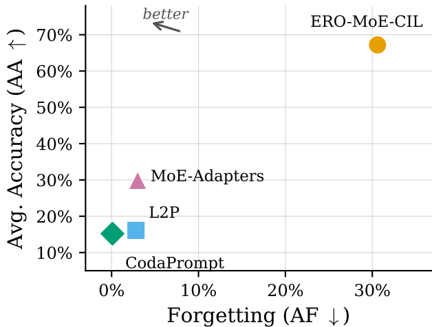
StateFarm
