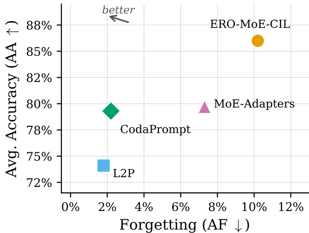
CIFAR-100
