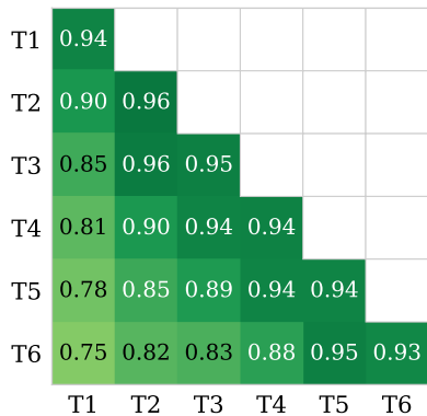
CIFAR-100
