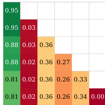
MoE-Adapters
