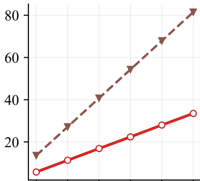
Threads=3
