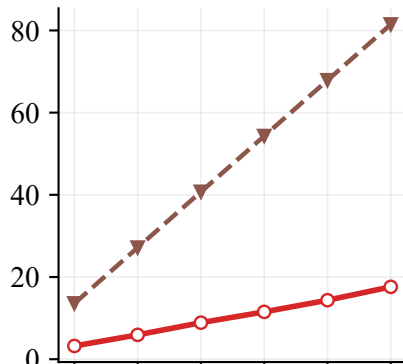
Threads=6
