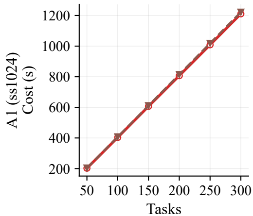
Threads=1
