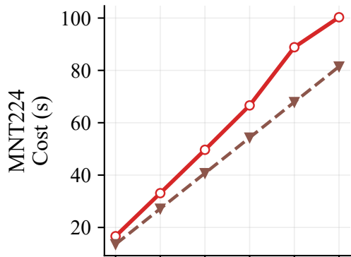
Threads=1
