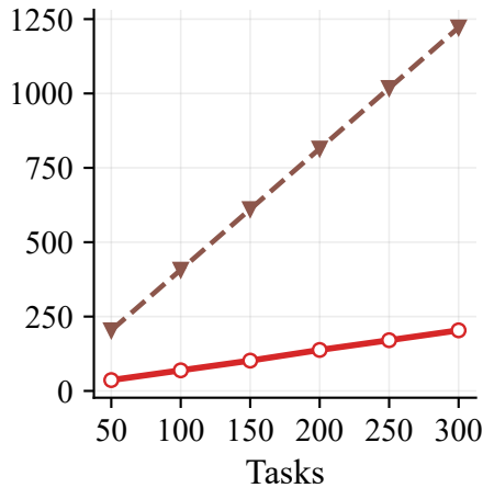
Threads=6
