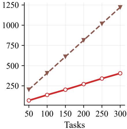
Threads=3
