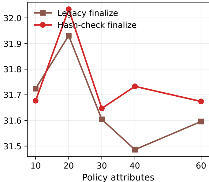
User finalize cost (ms)
