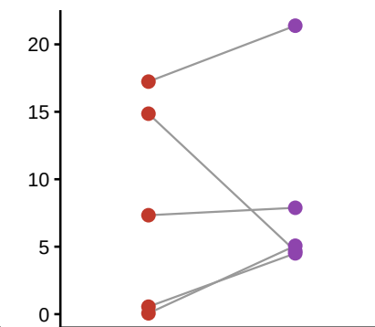
MMD z-score
