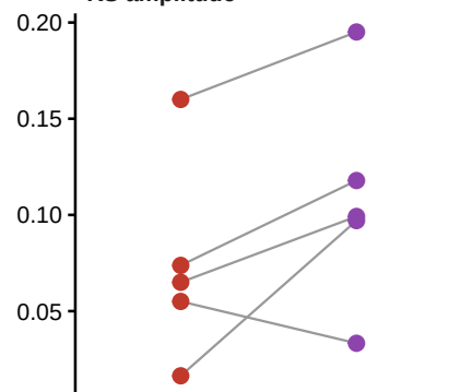
MMD envelope
