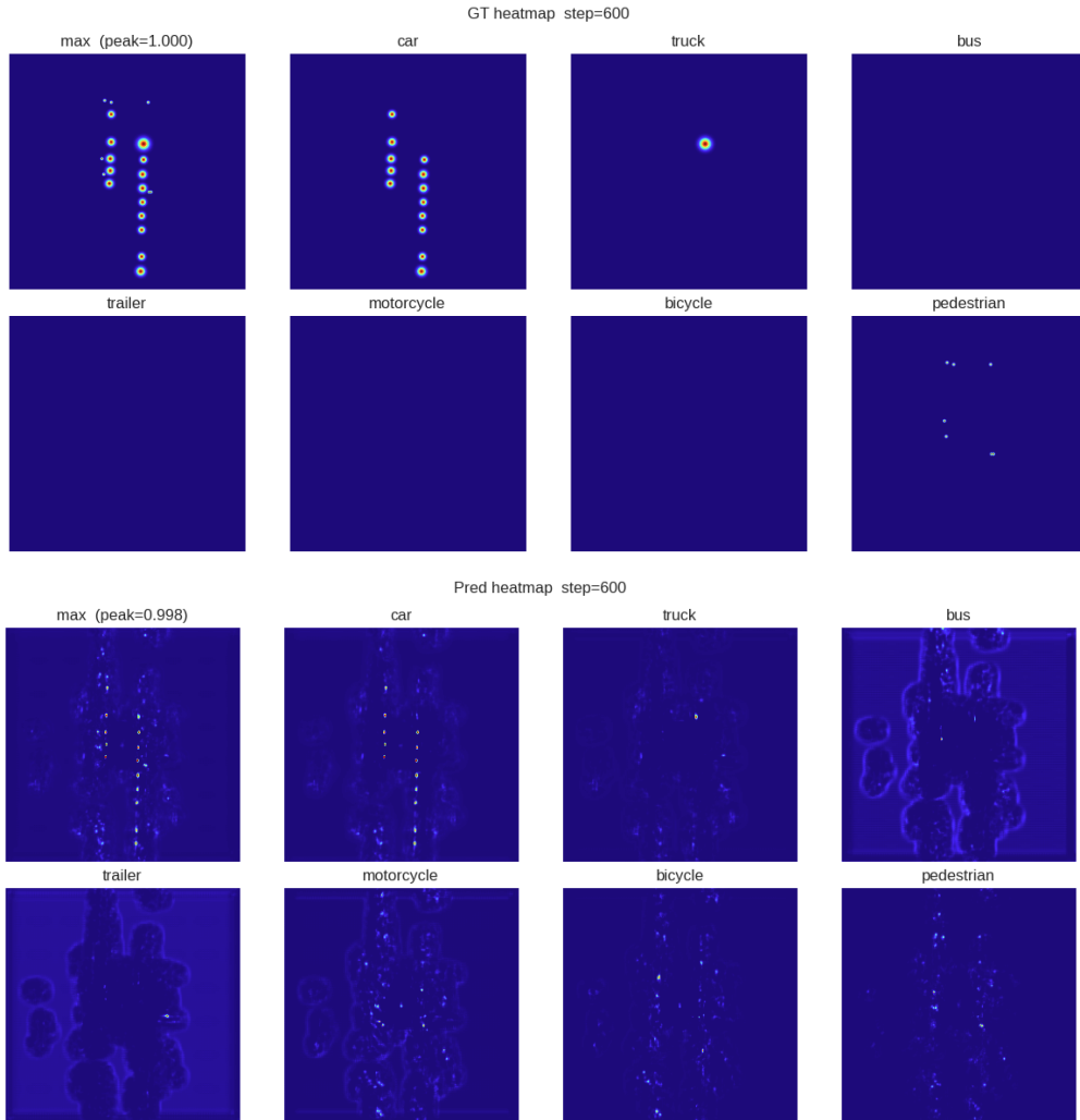
Figure 2.3: Ground-truth (top) and predicted (bottom) class-specific heatmap \hat{S} over the LiDAR BEV plane, stage 1 (LiDAR only), training step 600. Each panel shows the aggregate max channel plus one channel per class; probability mass is already concentrated on car and pedestrian , consistent with the per-class EPA/AMOTA breakdown in Tables 2.3 and 2.4.
