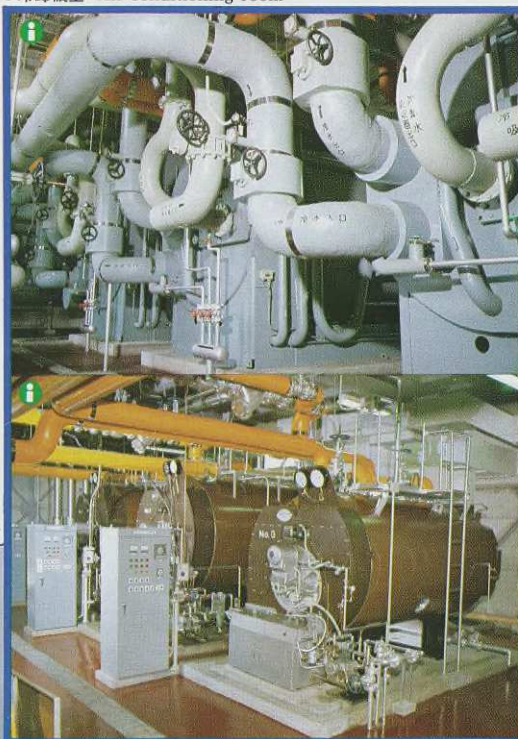
● 冷却機室 Air-conditioning room
