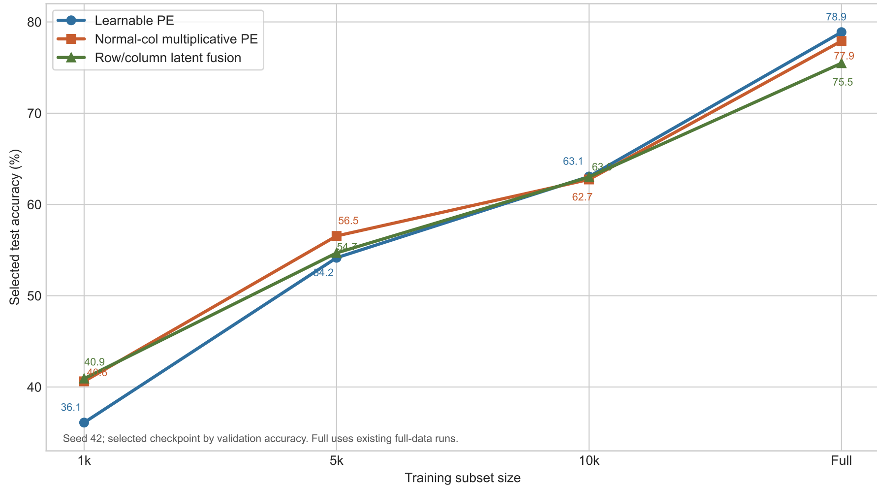
CIFAR-10 Low-Data vs Full-Data Positional Encoding Comparison
