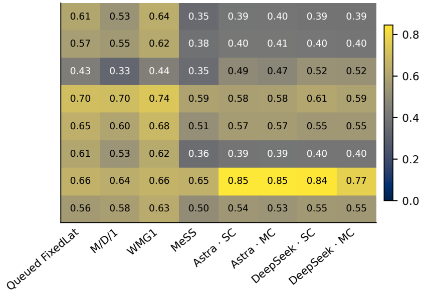
Request MAE/L
