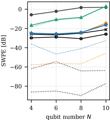
(a) depolarizing p = 0.01
