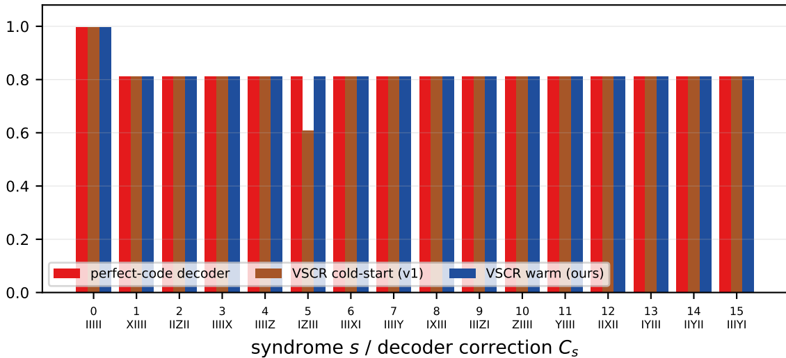
conditional fidelity cf_s
