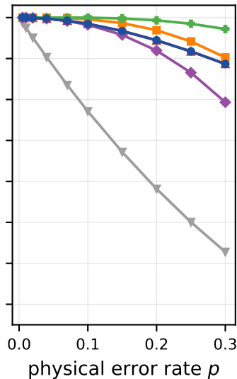
Amplitude damping
