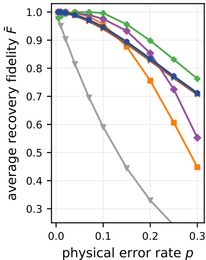
Depolarizing
