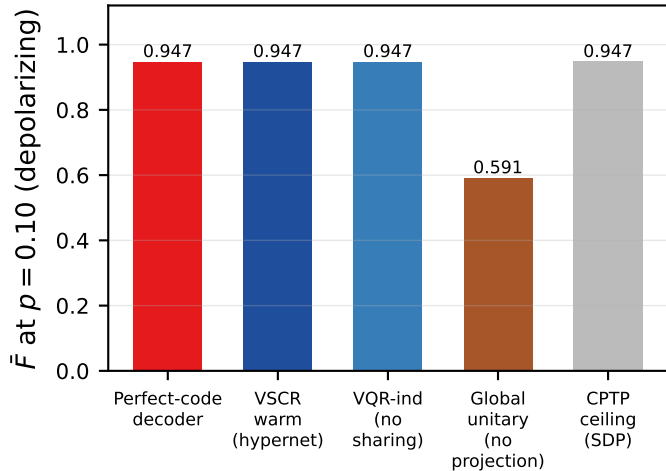
same-family baselines & CPTP ceiling
