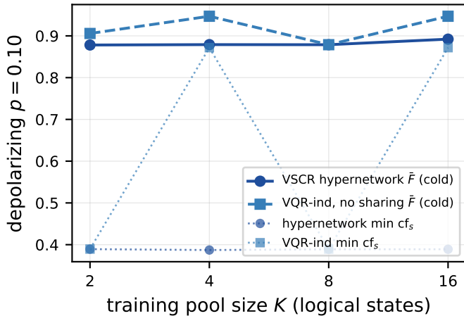
low-data regime (cold start)
