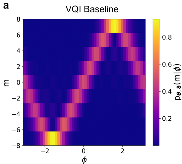
Quantum feature Heatmap
