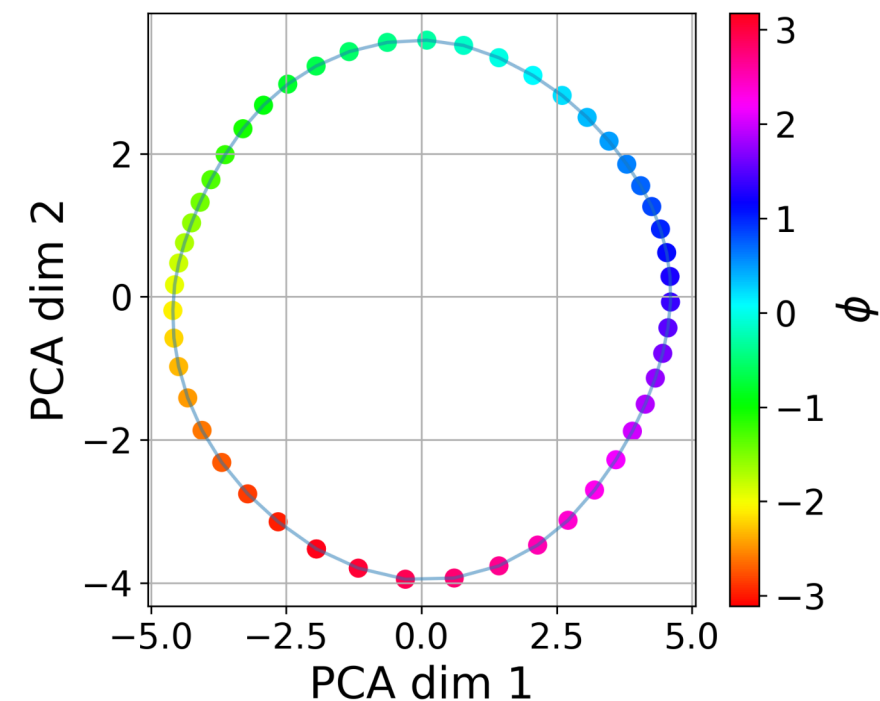
Arctan
