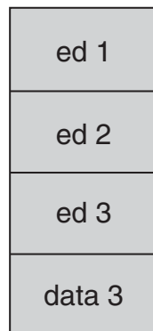
process P_3
