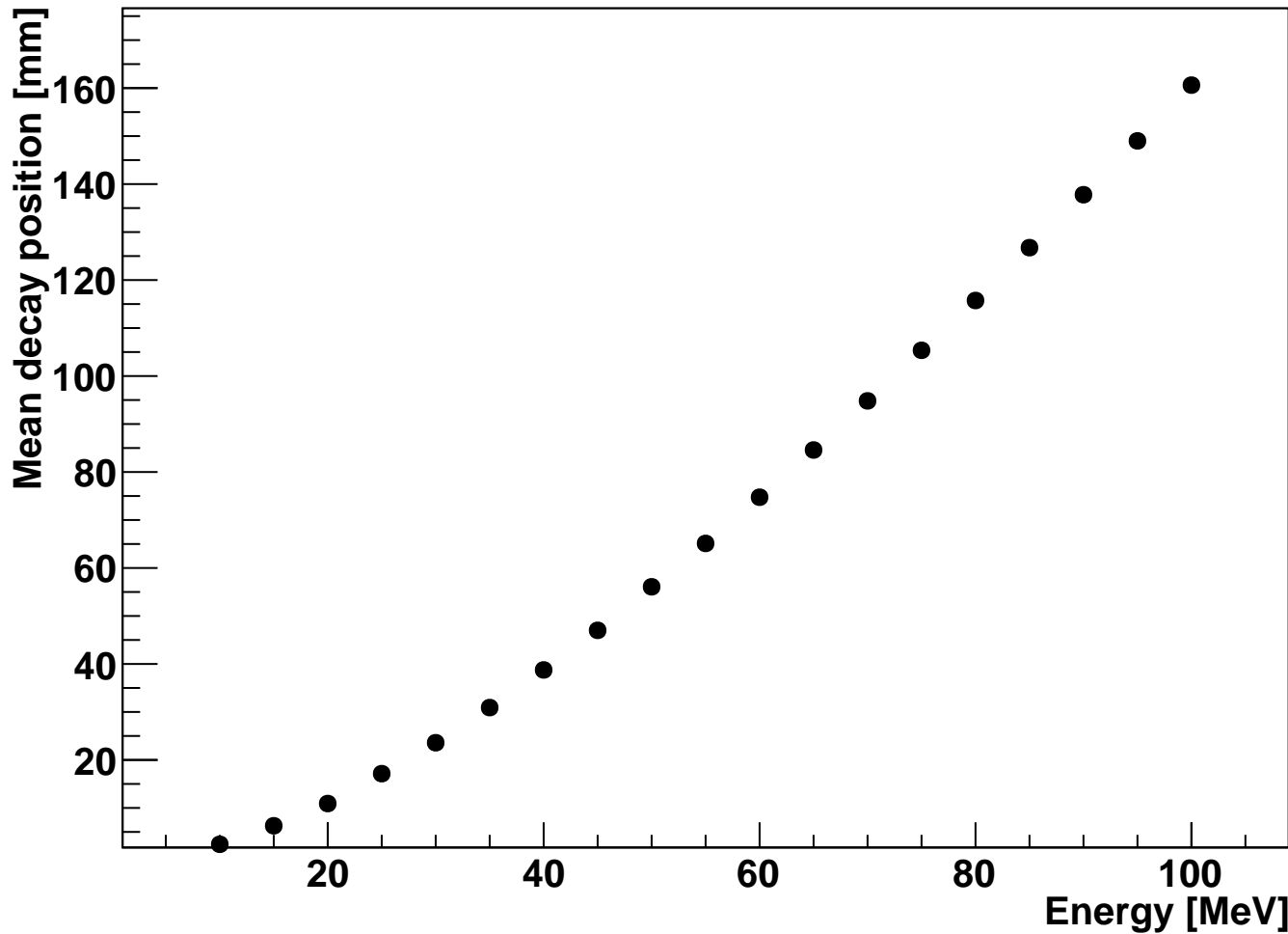
Mean decay position vs Energy (muons_B)
