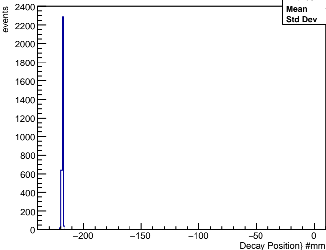
Z Position of Decay
