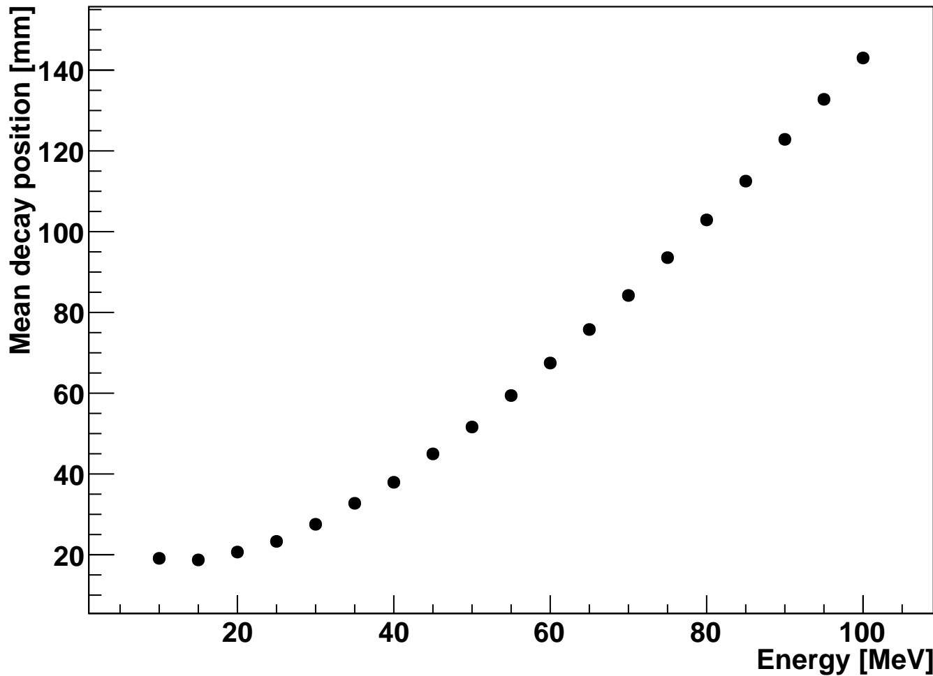
Mean decay position vs Energy (pions_B)
