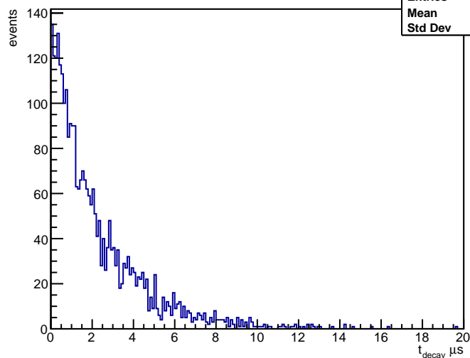
Time of Decay
