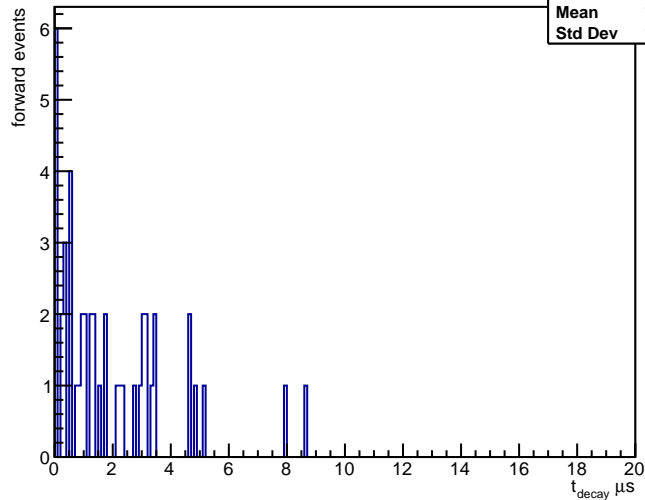
Time of Decay [Forward electron]
