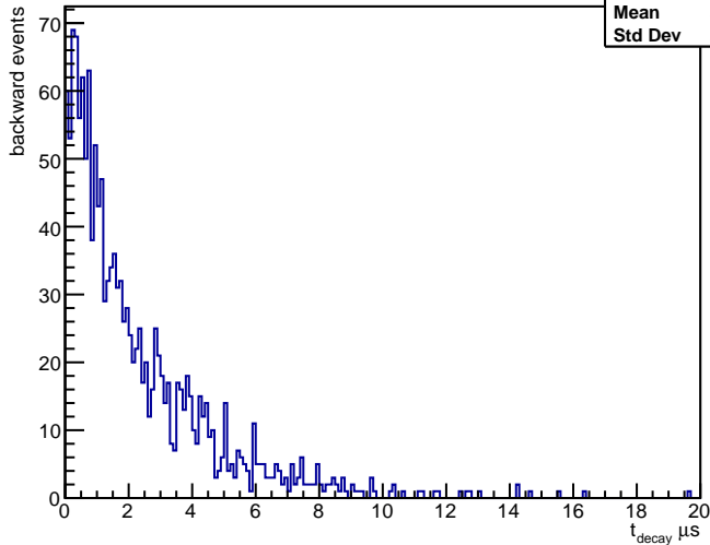
Time of Decay [Backward electron]
