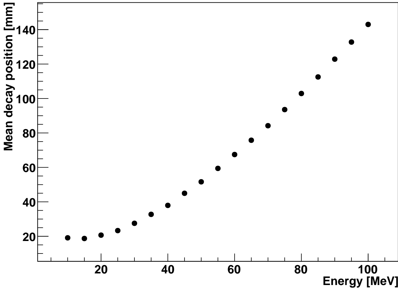
Mean decay position vs Energy (muons_noB)
