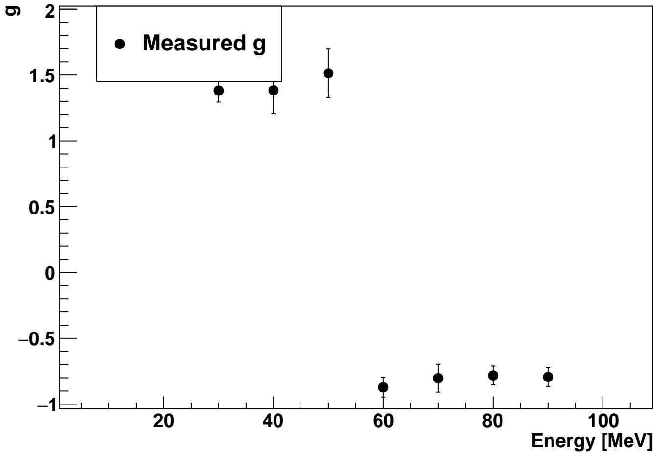
Pion g-factor vs Energy
