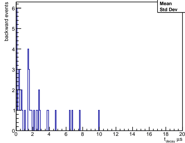
Time of Decay [Backward electron]
