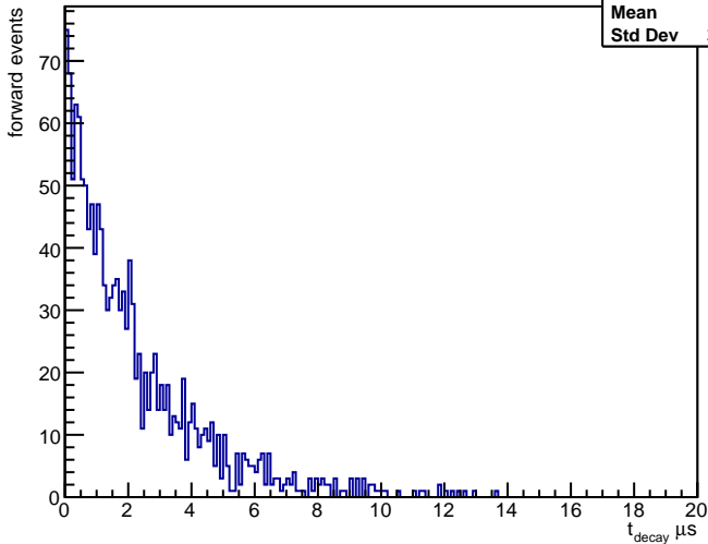
Time of Decay [Forward electron]
