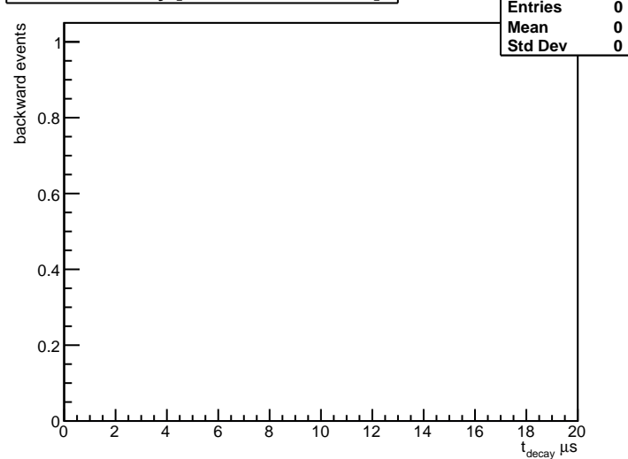
Time of Decay [Backward electron]
