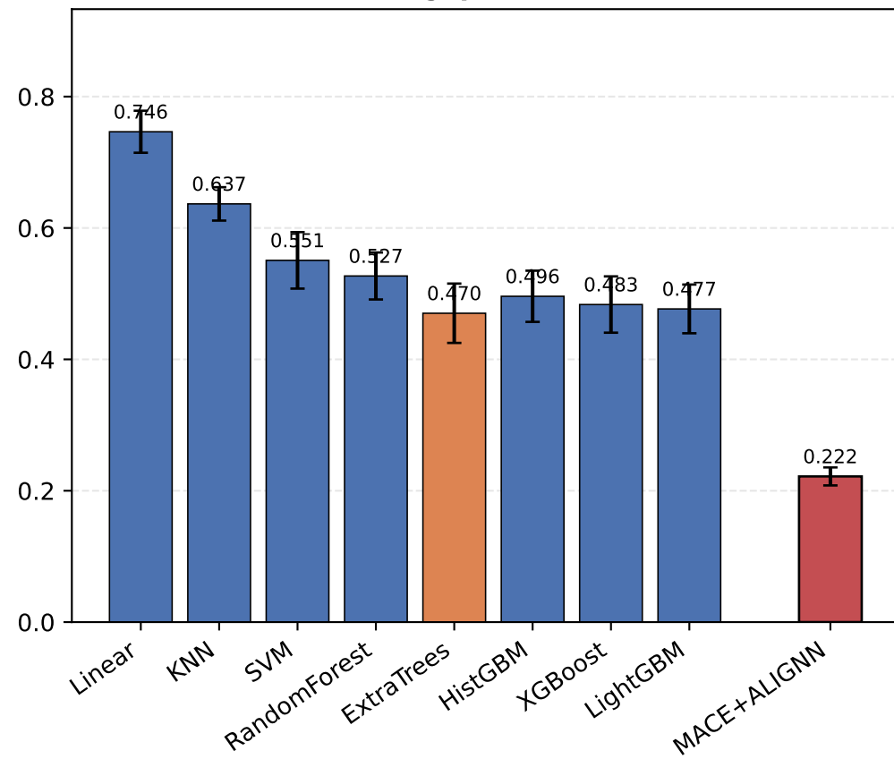
Bandgap MAE (eV)
