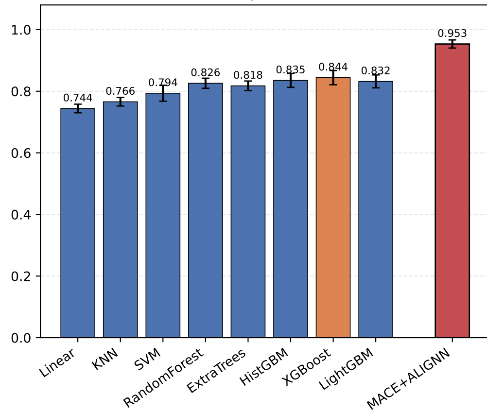
Stability macro-F1
