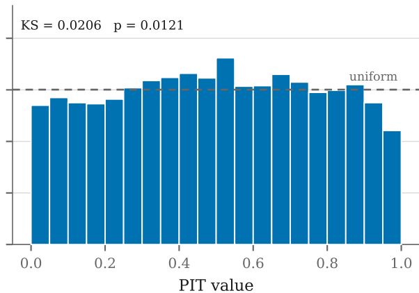
(b) Student-t + calibration
