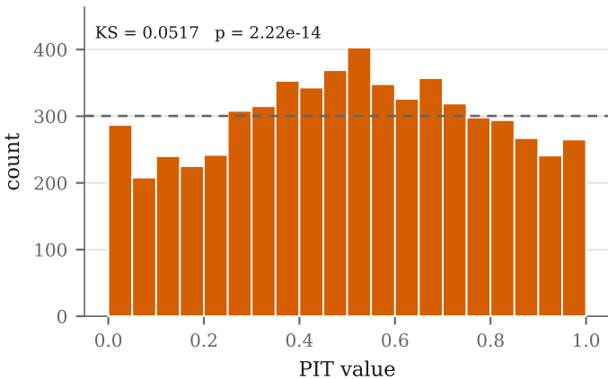
(a) Gaussian innovations
