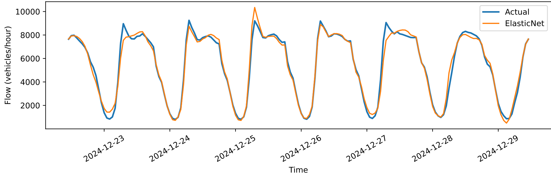
ElasticNet vs Actual — 12h horizon — station 3015021
