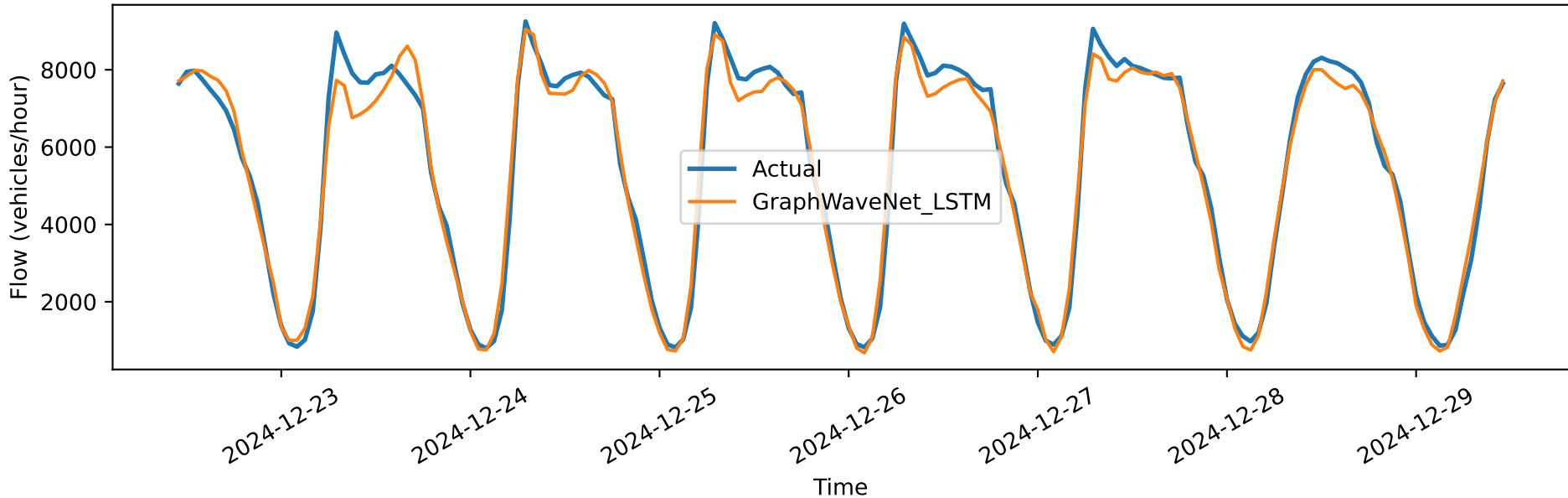
GraphWaveNet_LSTM vs Actual — 12h horizon — station 3015021
