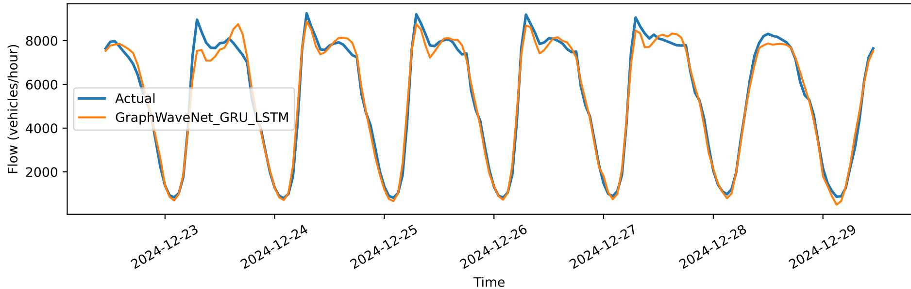
GraphWaveNet_GRU_LSTM vs Actual — 12h horizon — station 3015021
