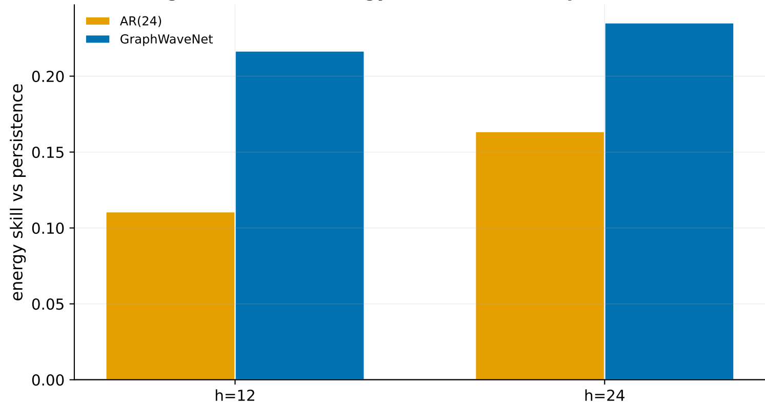
Figure 11. Wave-energy forecast skill (vs persistence)
