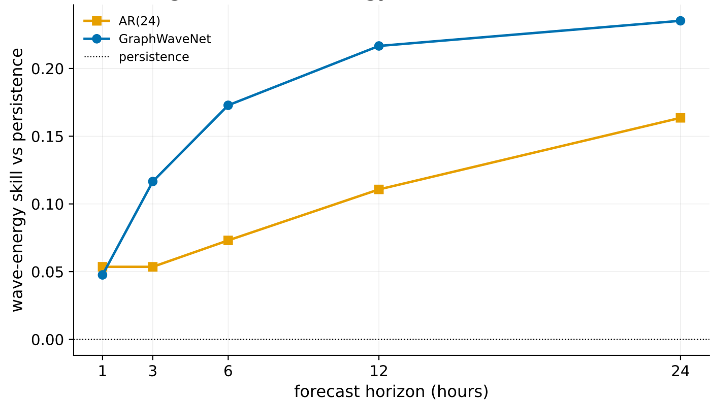
Figure 11. Wave-energy forecast skill vs horizon
