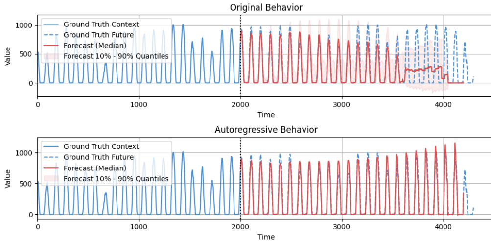
Figure 2: Comparison of autoregressive behavior vs. nan-filling method.
