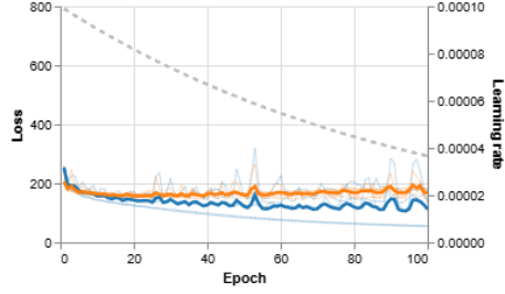
custom tirex | shift | slstm | mse
