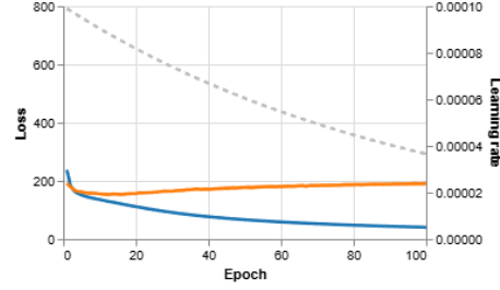
custom tirex | shift | lstm | mse
