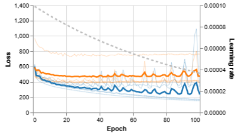
custom tirex | cpm | slstm | l1
