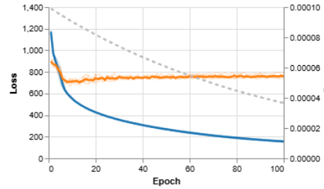
custom tirex | cpm | lstm | l1
