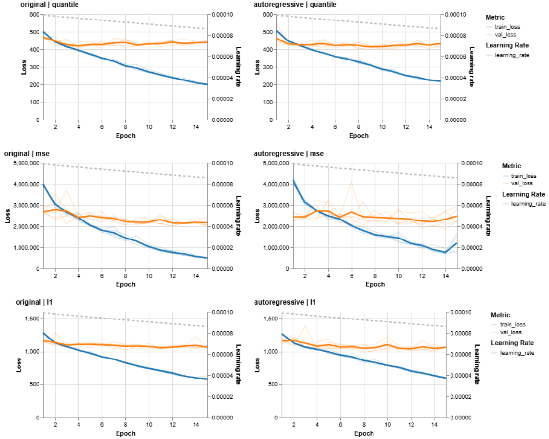
Training curves – all models (mean \pm individual runs)
