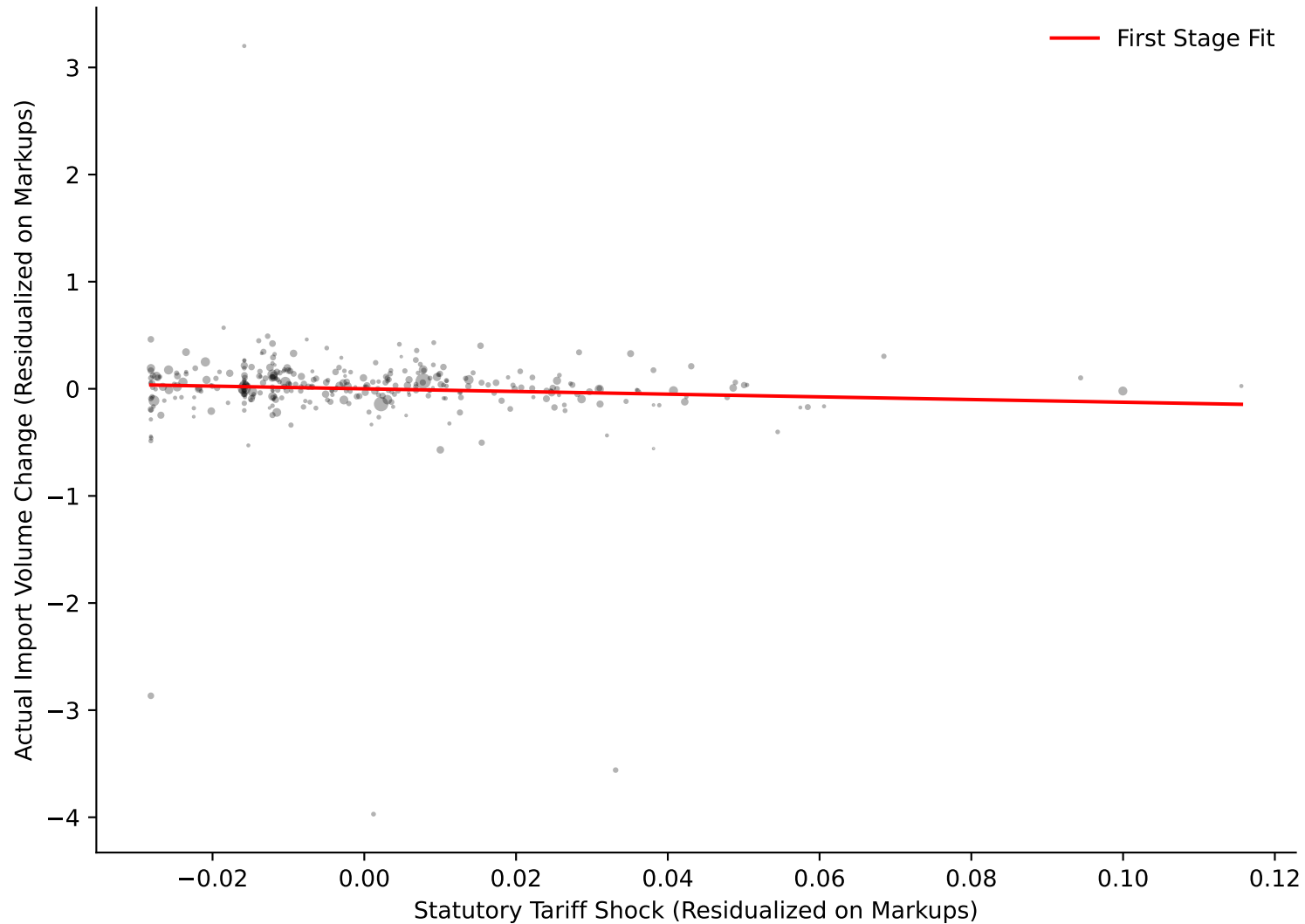
First-Stage Added Variable Plot (ADH Style)
