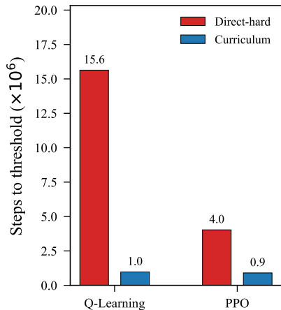
Environment steps to train Mountain Car on 2x Path Amplitude (representative run)
