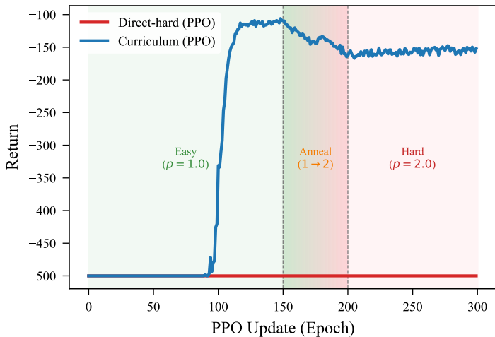
Learning curves for PPO on MountainCar varying Path Amplitude (representative run)
