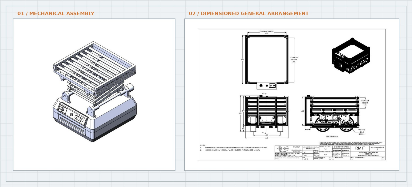
Selected academic work / assembly model and general arrangement drawing
