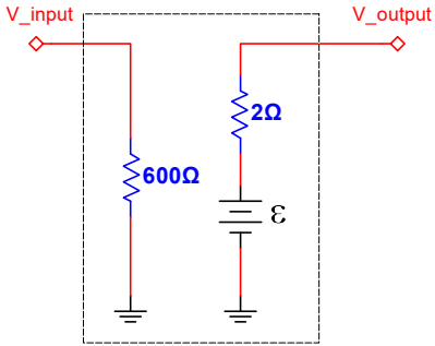
Audio amplifier
