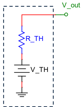
A "Thevenin equivalent circuit"
