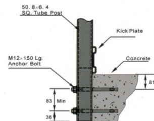
Drawing F-Side Mounted Post
