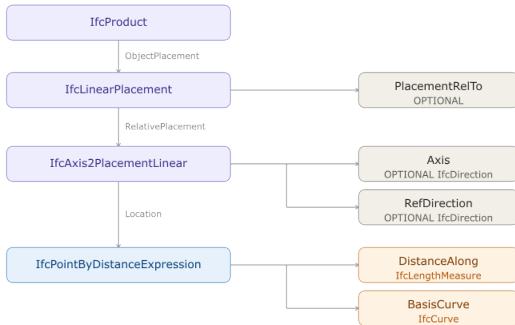
Figure 8.1.2-1 — IFC object graph for linear placement.
