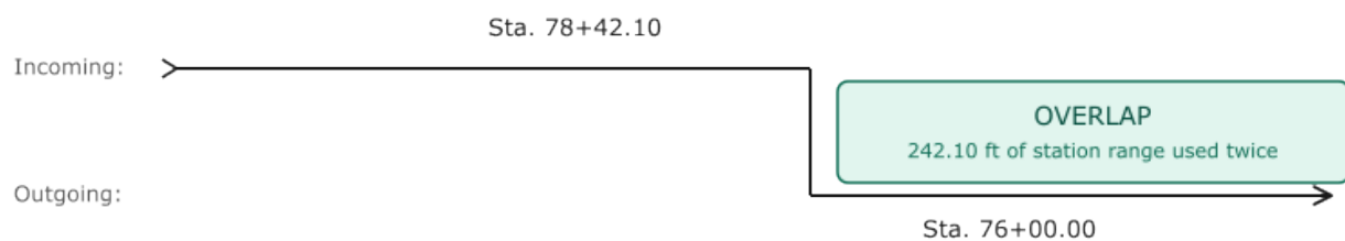
Figure 9.3.3-1 — Station overlap equation. Geometry is continuous; station numbers jump backward.
