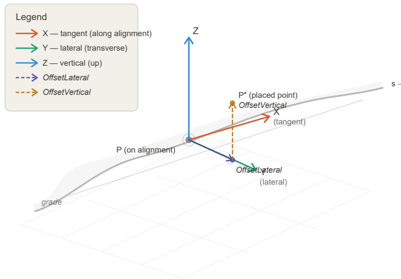
Figure 8.3.3-1 — Diagram showing the local coordinate system axes (X forward, Y left, Z up) at a point on a curved, graded alignment, with annotations for DistanceAlong, OffsetLateral, and OffsetVertical.
