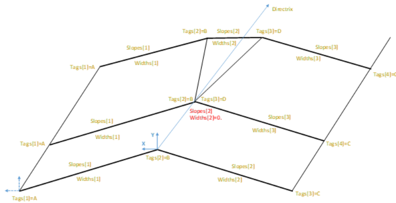
Figure 10.3.1-1 — Sectioned surface with breaklines at cross-section topology changes. (source bSI)
