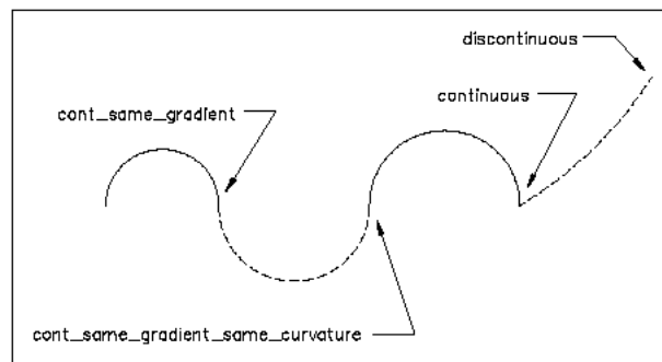
Figure 11.0-1 - Illustration of segment transition types
