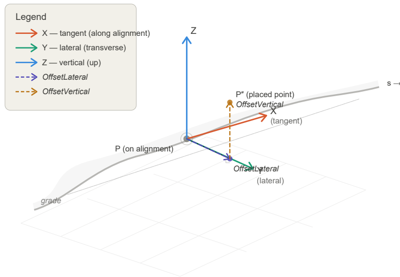
Figure 6.3.3-1 — Diagram showing the local coordinate system axes ( X forward, Y left, Z up) at a point on a curved, graded alignment, with annotations for DistanceAlong, OffsetLateral, and OffsetVertical.
