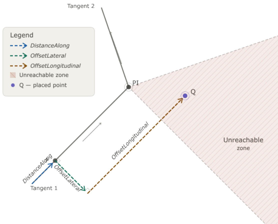
Figure 8.2.1.4.1-1 — Plan view showing two tangent lines meeting at an angle point (PI). The shaded region outside the angle cannot be reached by a station + lateral offset alone. An object in this region requires a longitudinal offset.
