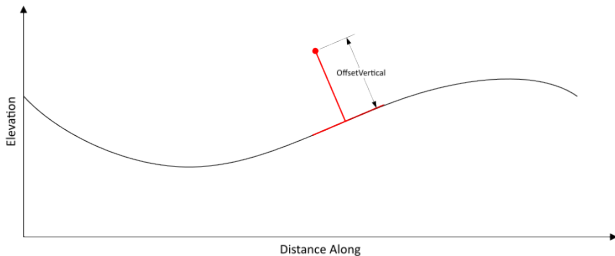
Figure 8.2.1.3-1 — Elevation view of an alignment profile showing the OffsetVertical in the positive sense.
