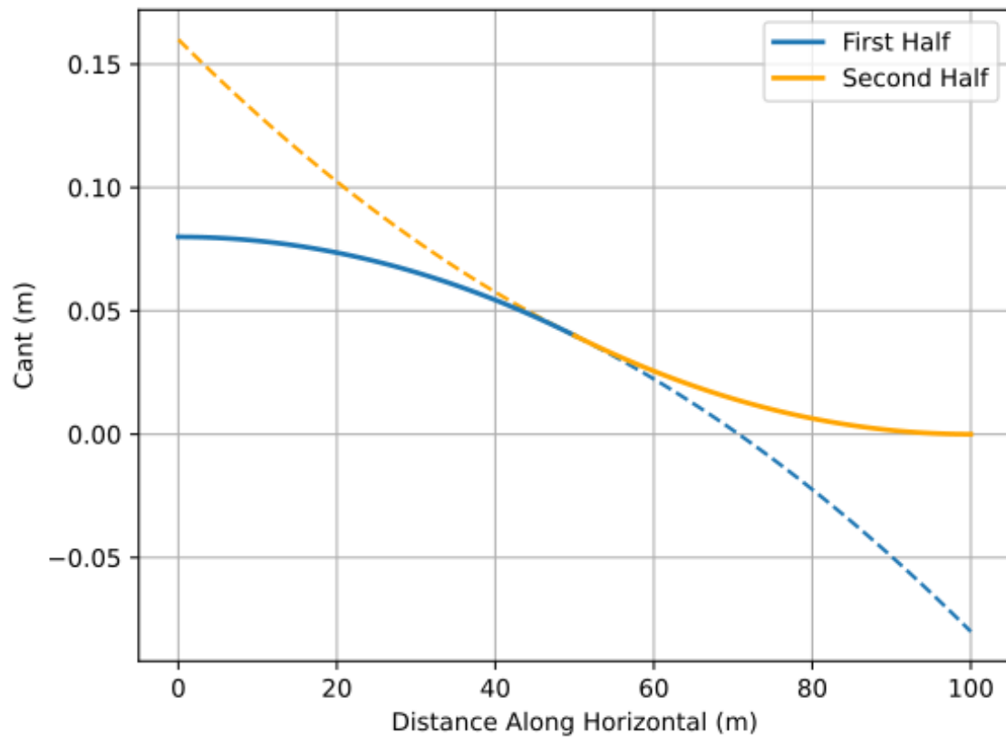
Figure 4.5.2-1 - IfcSecondOrderPolynomialSpiral parent curves. The dashed lines represent the projection of the parent curve over the full length of the segment.
