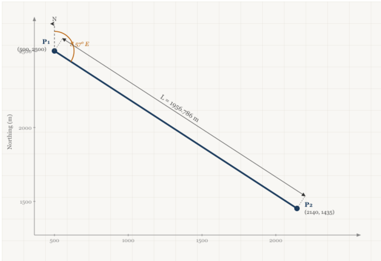
Figure 2.3.2-1 Tangent segment
