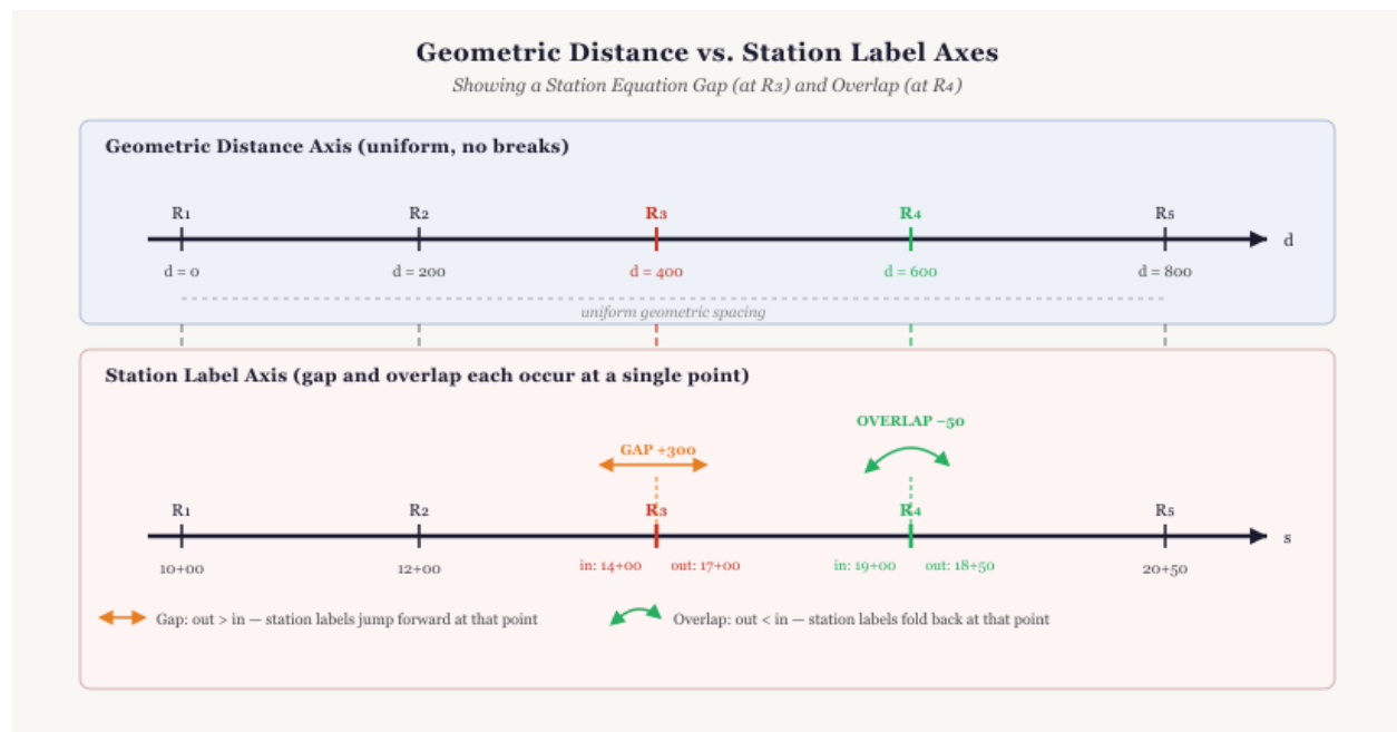
Figure 9.3.4-1 — Two-axis diagram comparing DistanceAlong (geometric distance) and station label for an alignment with one gap equation and one overlap equation.
