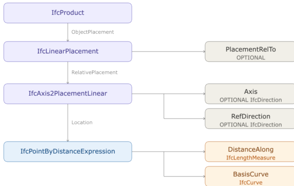
Figure 8.1.2-1 — IFC object graph for linear placement.
