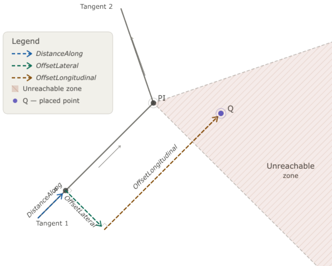
Figure 8.4.1-1 — Plan view showing two tangent lines meeting at an angle point (PI). The shaded region outside the angle cannot be reached by a station + lateral offset alone. An object in this region requires a longitudinal offset.
