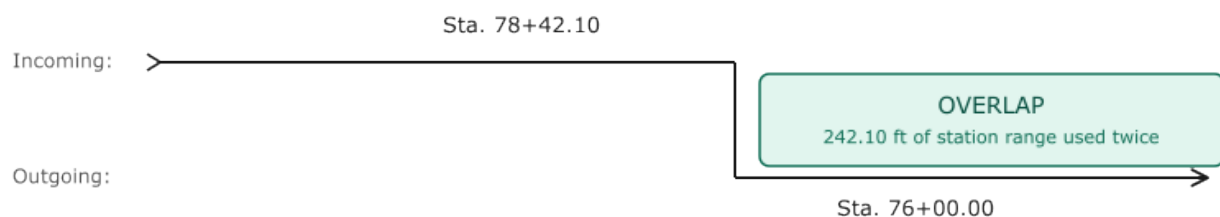
Figure 9.3.3-1 — Station overlap equation. Geometry is continuous; station numbers jump backward.
