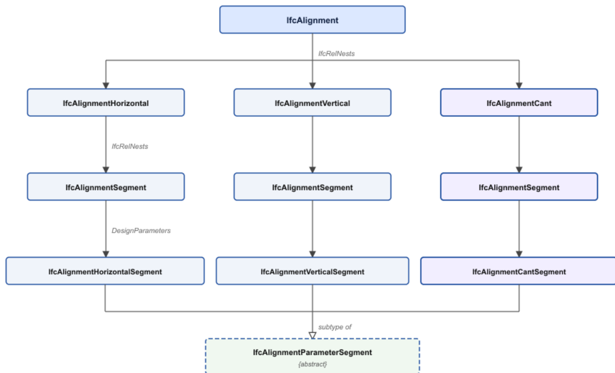
Figure 1.4-1 Semantic alignment model
