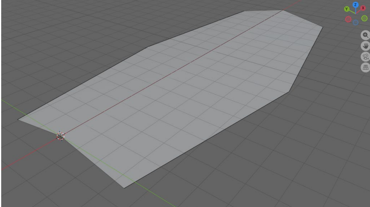
Figure 10.6.1.4-1 — Expected geometry of IfcSectionedSurface with stringline guide curves. This rendering has been synthesised to illustrate the correct geometry; no viewer capable of resolving stringline guide curves has been found at the time of writing.
