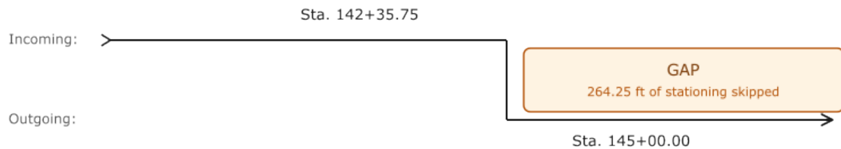
Figure 9.3.2-1 — Station gap equation. Geometry is continuous; station numbers jump forward.
