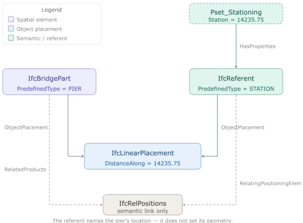
Figure 9.5.2-1 — Object graph showing an IfcBridgePart.PIER with its own IfcLinearPlacement , an IfcReferent ( STATION type) with Pset_Stationing , and the IfcRelPositions link between them.
