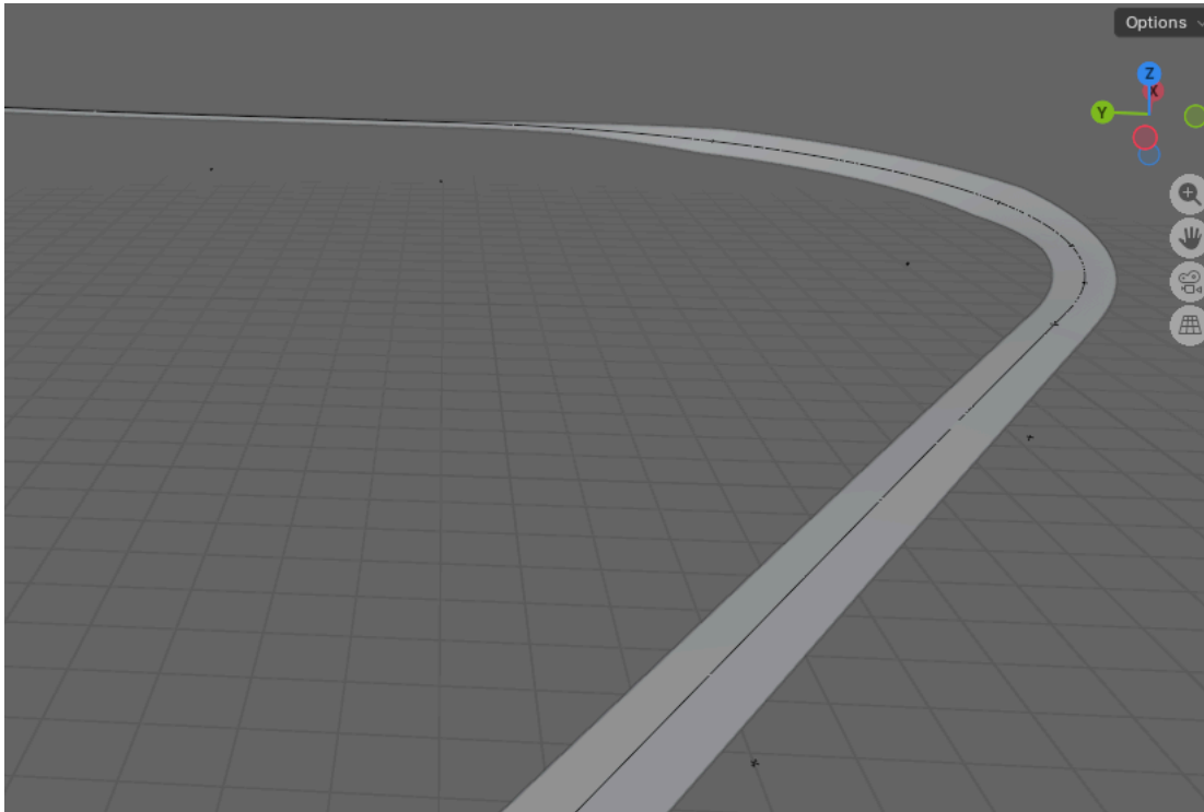
Figure 8.1-1 Superelevation transition
