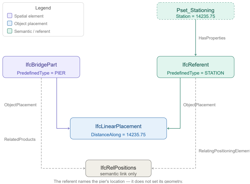
Figure 7.5.2-1 — Object graph showing an IfcBridgePart.PIER with its own IfcLinearPlacement , an IfcReferent ( STATION type) with Pset_Stationing , and the IfcRelPositions link between them. Annotate that the referent provides the station label; it does not set the geometry.
