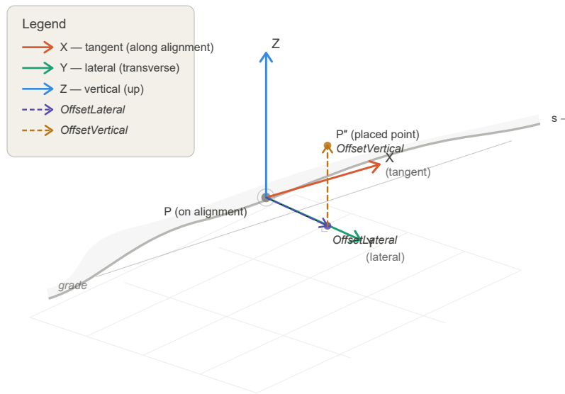
Figure 5.3.3-1 — Diagram showing the local coordinate system axes (X forward, Y left, Z up) at a point on a curved, graded alignment, with annotations for DistanceAlong, OffsetLateral, and OffsetVertical.
