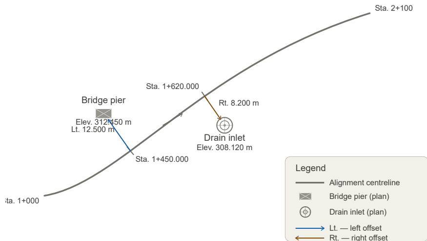
Figure 5.1.2-1 — Conceptual diagram showing a plan view of an alignment with a bridge pier placed at a station/offset and a drain inlet placed at station/offset/elevation.
