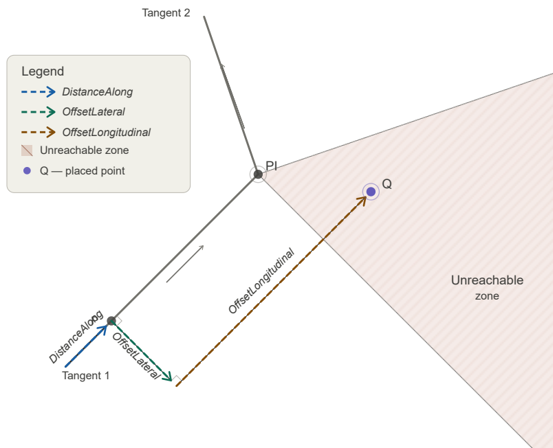
Figure 5.4.1-1 — Plan view showing two tangent lines meeting at an angle point (PI). The shaded region outside the angle cannot be reached by a station + lateral offset alone. An object in this region requires a longitudinal offset.
