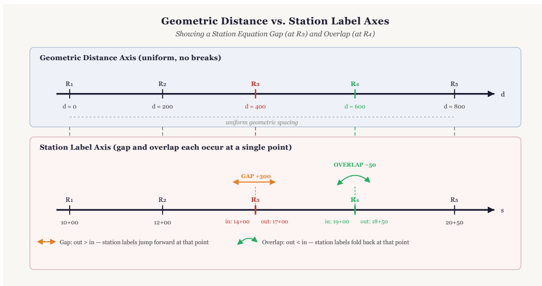
Figure 7.3.4-1 — Diagram showing a timeline of DistanceAlong (geometric) vs. station label for an alignment with one gap equation and one overlap equation. Annotate the start station, equation points, and the non-linear relationship between station and distance.
