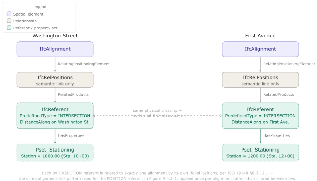
Figure 9.5-1 — Two independent INTERSECTION referents, each related to its own alignment by its own IfcRelPositions , following the same alignment-link pattern as the POSITION referent in Figure 9.4.2-1 — applied once per alignment rather than shared between two.
