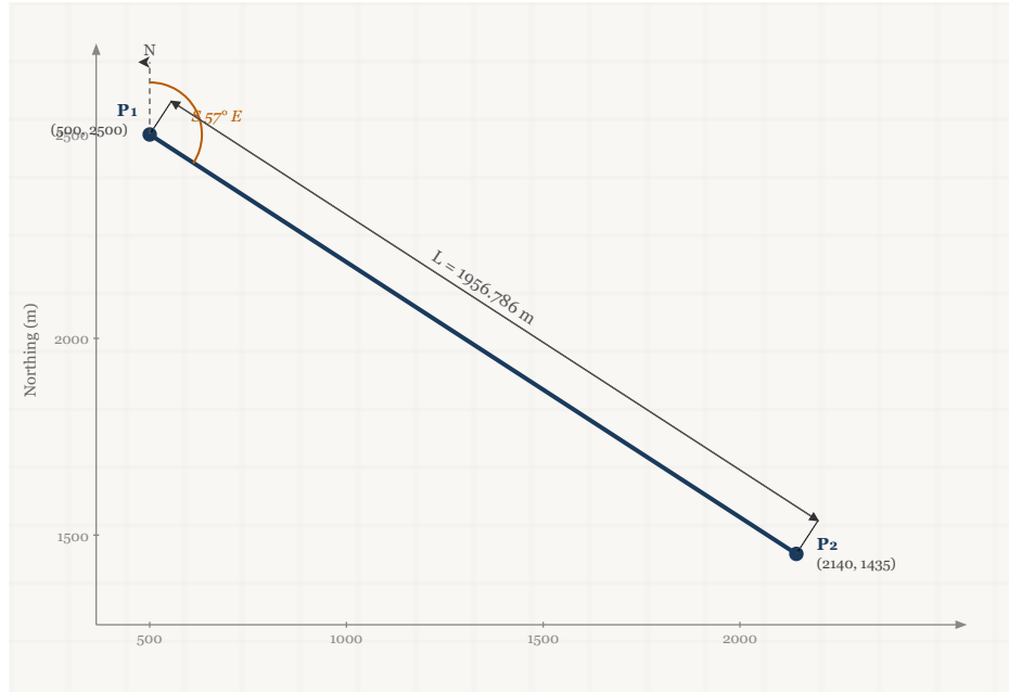
Figure 2.3.2-1 Tangent segment
