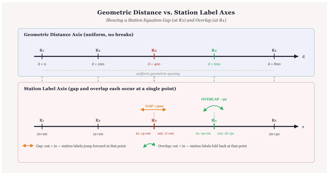
Figure 7.3-3 — Diagram showing a timeline of DistanceAlong (geometric) vs. station label for an alignment with one gap equation and one overlap equation. Annotate the start station, equation points, and the non-linear relationship between station and distance.
