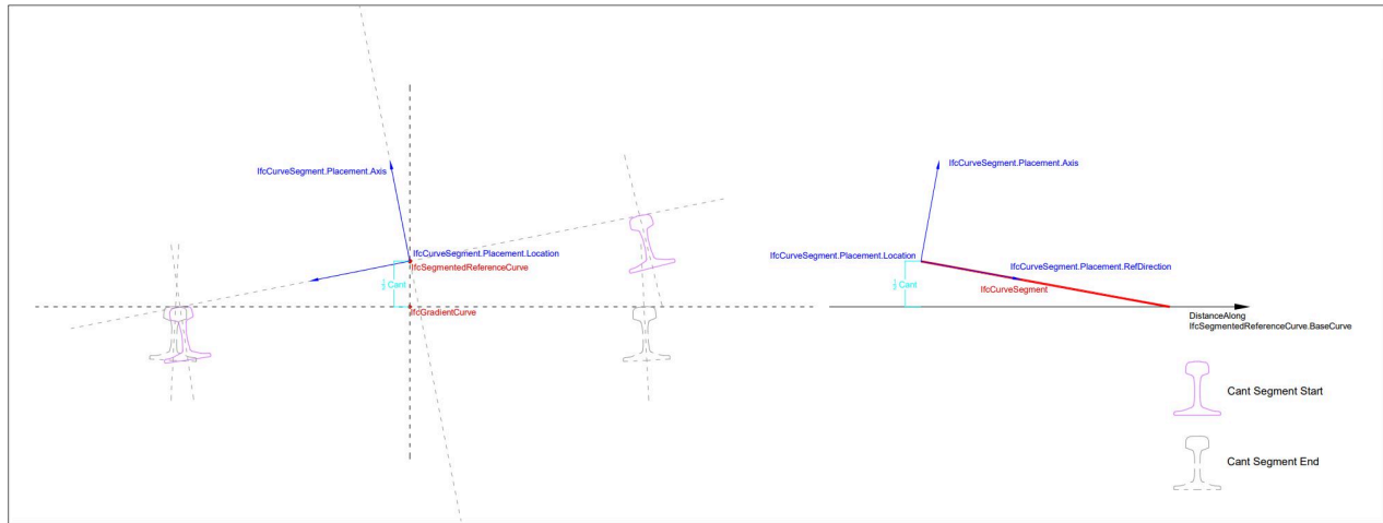
Figure 4.1.1-1 - cross section and elevation of a cant segment (source: bSI)
