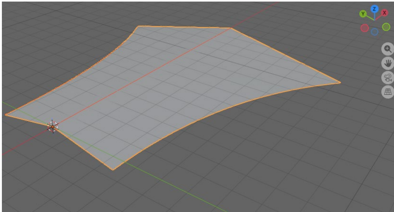
Figure 10.6.1.6-2 — Expected geometry of IfcSectionedSurface_with_stringlines_independent_edge_alignments.ifc . This rendering has been synthesized to illustrate the correct geometry; no viewer capable of resolving string line guide curves has been found at the time of writing.
