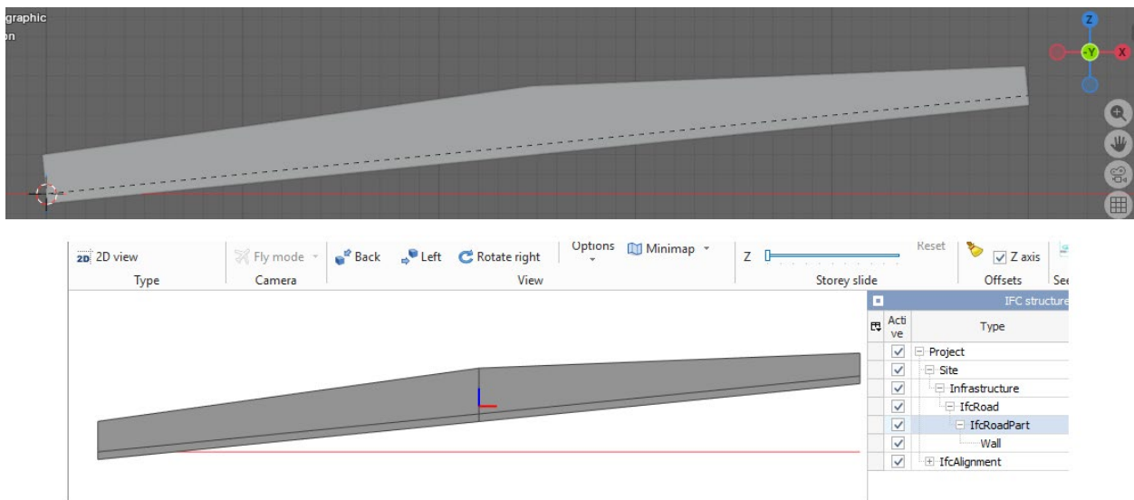
Figure 10.5.5-2 — The same IfcSectionedSolidHorizontal model (retaining wall, 10% grade, Axis omitted) rendered by two IFC viewers: the upper half assumes Axis perpendicular to the 3D tangent (inclined end face); the lower half assumes Axis = (0, 0, 1) (plumb end face).
