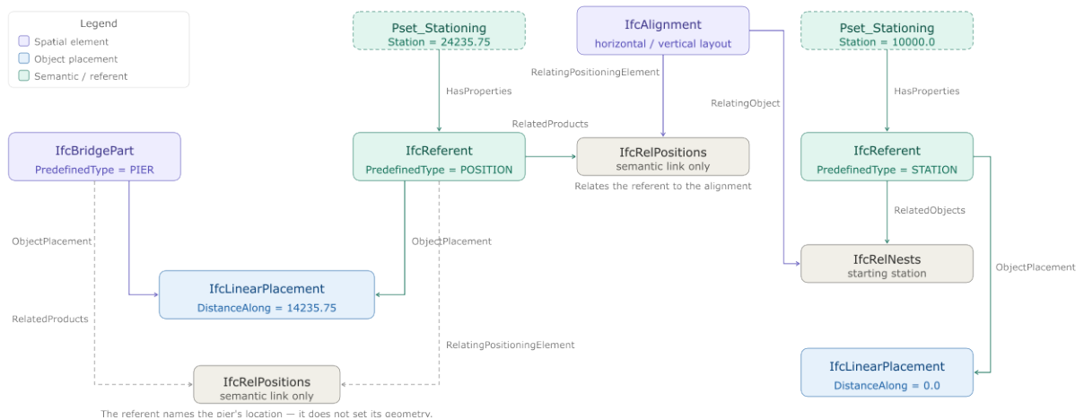
Figure 9.4.2-1 — Object graph showing an IfcBridgePart.PIER with its own IfcLinearPlacement , an IfcReferent (POSITION type) with Pset_Stationing , and the IfcRelPositions link between them. To the right, IfcAlignment is the RelatingPositioningElement for a second IfcRelPositions that has the pier's referent as RelatedProducts , and a starting-station IfcReferent (Station = 10000.0) is nested under
