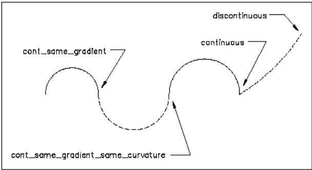
Figure 10.0-1 - Illustration of segment transition types
