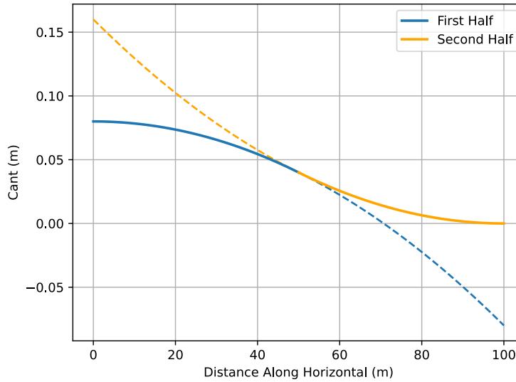
Figure 4.5.2-1 - IfcPolygonalSpiralCurve parent curves. The dashed lines represent the projection of the parent curve over the full length of the semantic segment.
