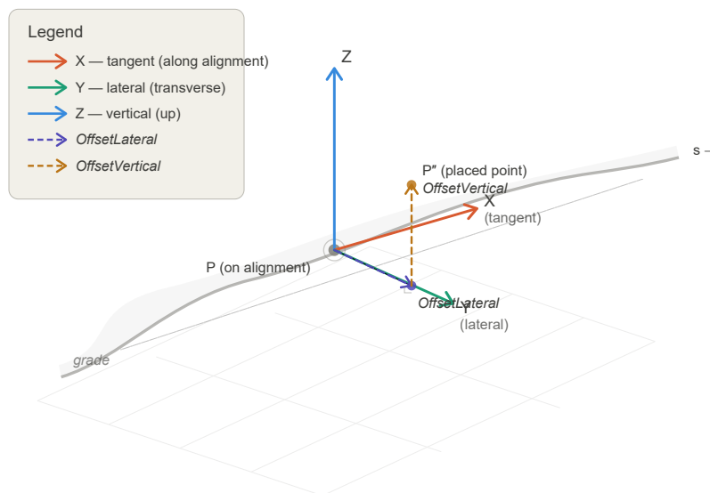
Figure 5.3.3-1 — Diagram showing the local coordinate system axes (X forward, Y left, Z up) at a point on a curved, graded alignment, with annotations for DistanceAlong , OffsetLateral , and OffsetVertical .
