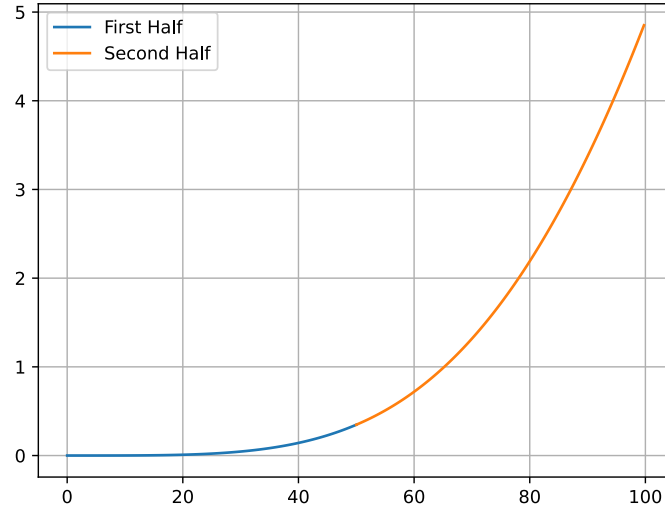
Figure 2.7.2-3 - Final Helmert transition curve
