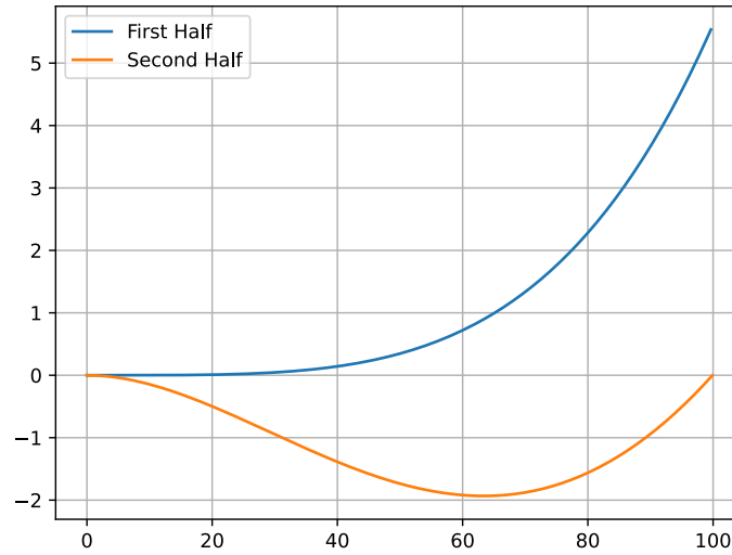
Figure 2.7.2-1 First and second half of parent curves, without placement adjustments
