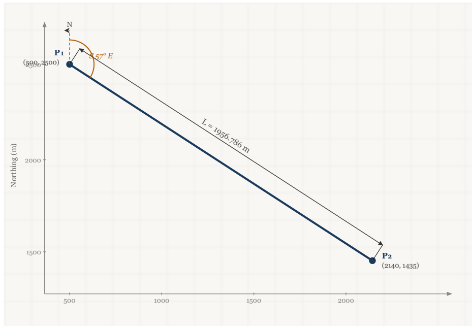
Figure 2.3.2-1 Tangent segment
