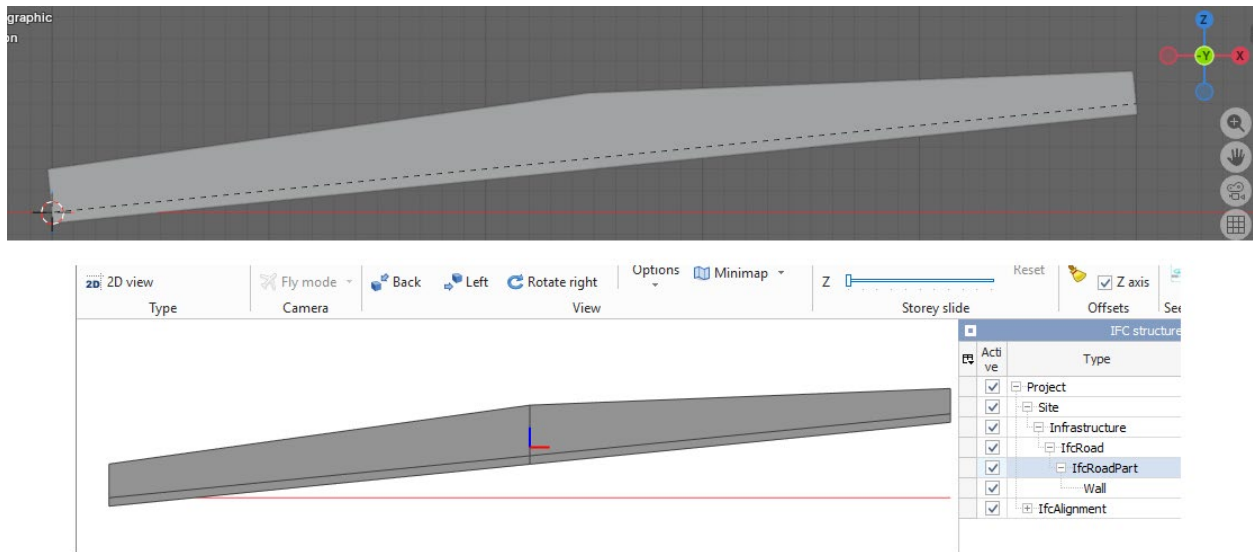
Figure 10.5-2 — The same IfcSectionedSolidHorizontal model (retaining wall, 10% grade, Axis omitted) rendered by two IFC viewers: upper half assumes Axis perpendicular to the 3D tangent (inclined end face); lower half assumes Axis = (0,0,1) (plumb end face).
