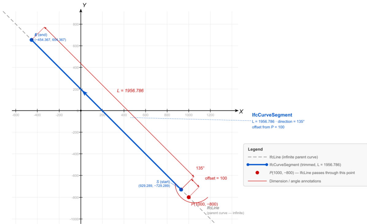
Figure 2.3.2-2 IfcLine at arbitrary placement
