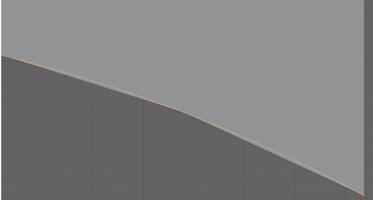
Figure 10.6.6-2 — Zoomed view of the far-right corner showing the gap between the piecewise-linear surface edge and the exact circular arc guide curve (orange). The error is largest at the midpoint between cross-sections.
