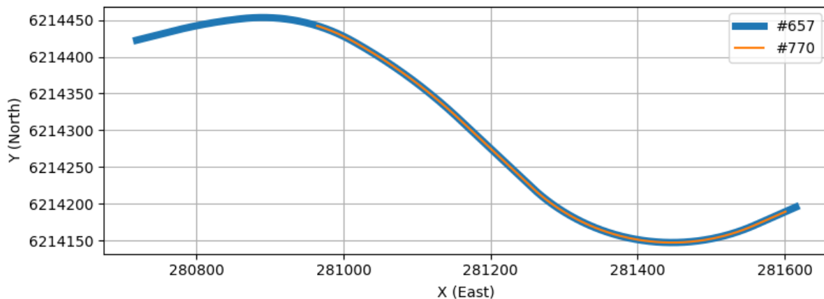
Figure 1.5.2-4 — Example of IfcGradientCurve with a start location and length different than the IfcCompositeCurve BaseCurve.
